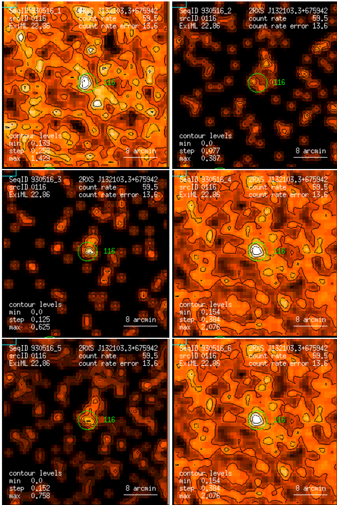
Figure 116: RASS 930516: detection 0116: band rate images, Gaussian filter: (1) PSPC channels 11 – 41, (2) 52 – 90, (3) 91 – 201, (4) 11 – 235, (5) 52 – 201, (6) 11 – 201. Broad band rates in counts/ks. Band rate contour levels in counts/ks/arcmin 2 .
