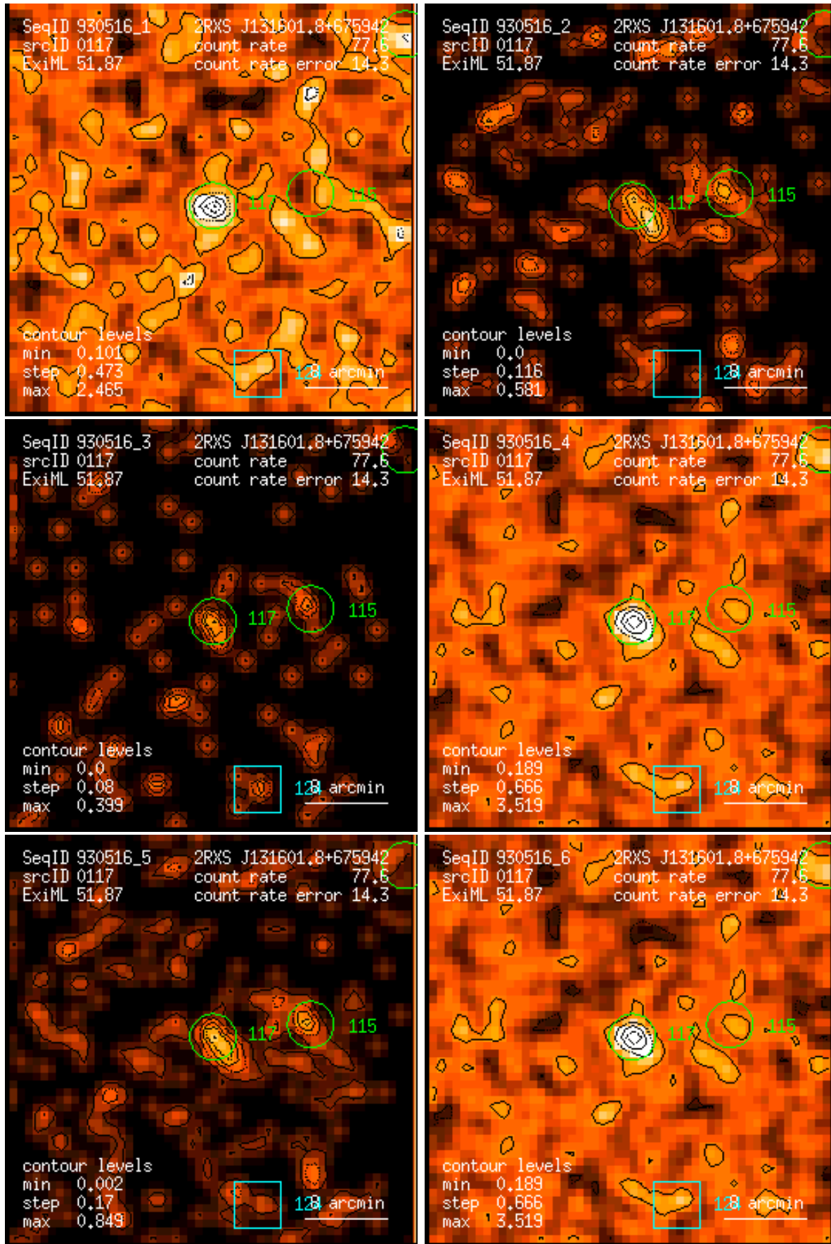
Figure 117: RASS 930516: detection 0117: band rate images, Gaussian filter: (1) PSPC channels 11 – 41, (2) 52 – 90, (3) 91 – 201, (4) 11 – 235, (5) 52 – 201, (6) 11 – 201. Broad band rates in counts/ks. Band rate contour levels in counts/ks/arcmin 2 .
