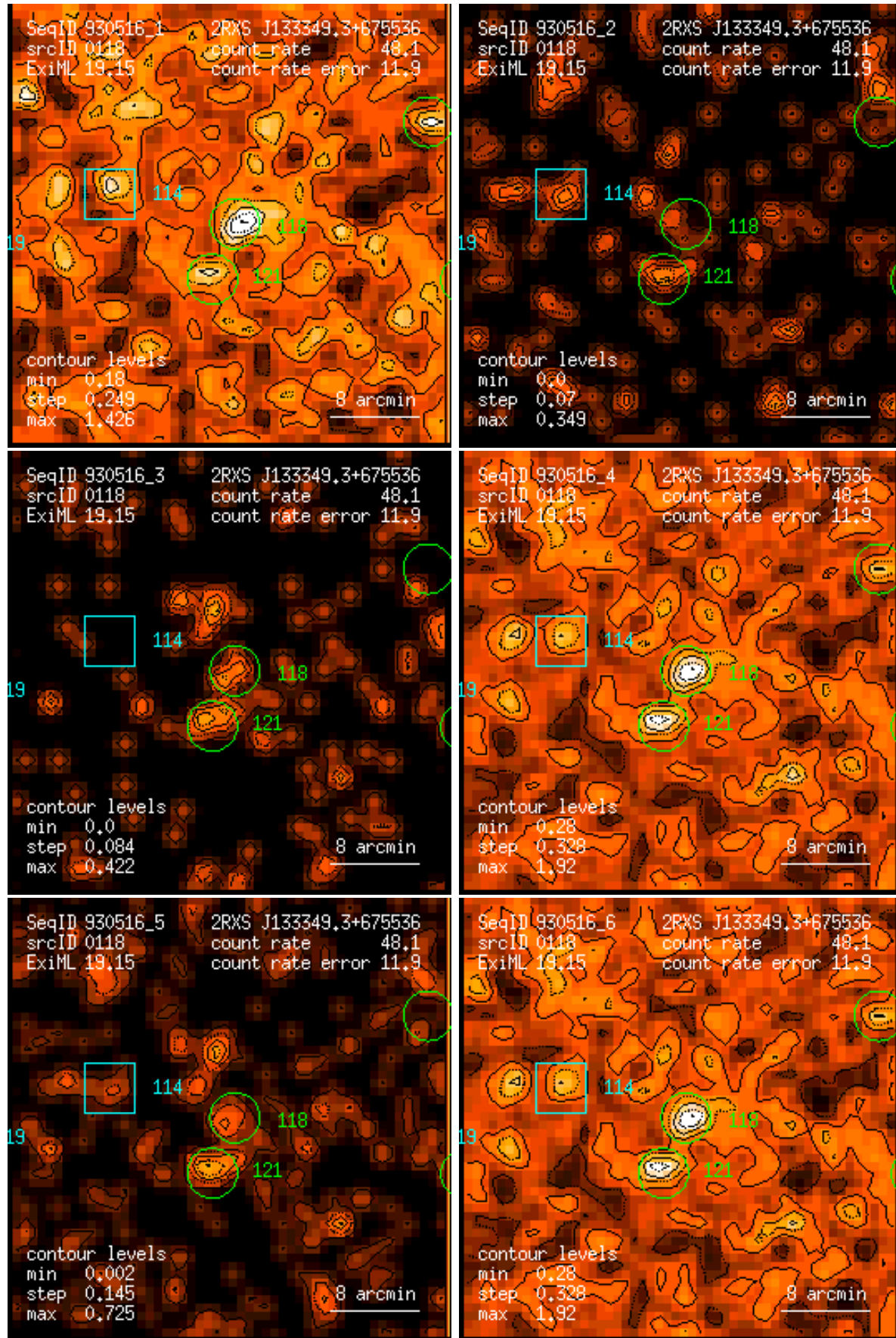
Figure 118: RASS 930516: detection 0118: band rate images, Gaussian filter: (1) PSPC channels 11 – 41, (2) 52 – 90, (3) 91 – 201, (4) 11 – 235, (5) 52 – 201, (6) 11 – 201. Broad band rates in counts/ks. Band rate contour levels in counts/ks/arcmin 2 .
