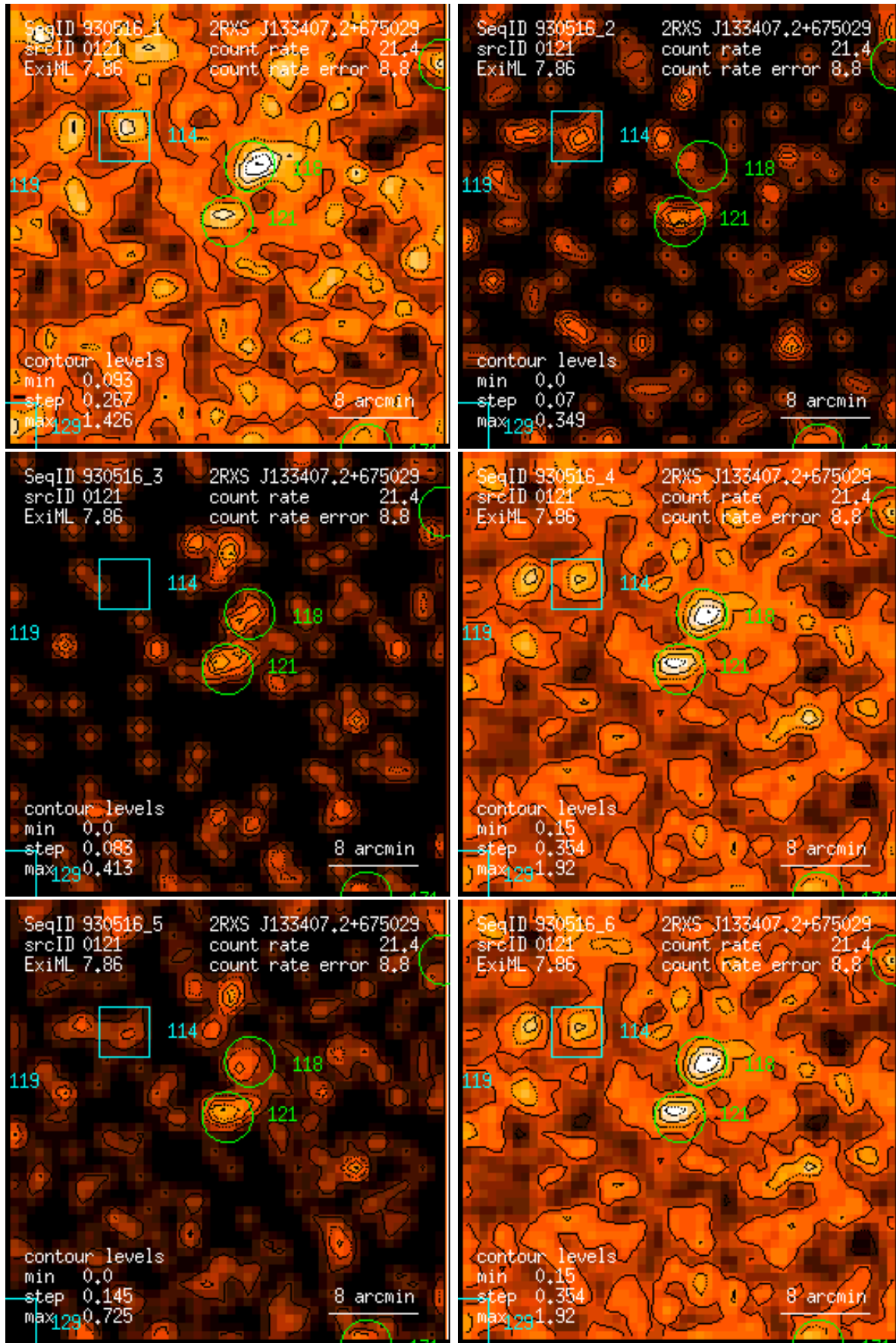
Figure 121: RASS 930516: detection 0121: band rate images, Gaussian filter: (1) PSPC channels 11 – 41, (2) 52 – 90, (3) 91 – 201, (4) 11 – 235, (5) 52 – 201, (6) 11 – 201. Broad band rates in counts/ks. Band rate contour levels in counts/ks/arcmin 2 .
