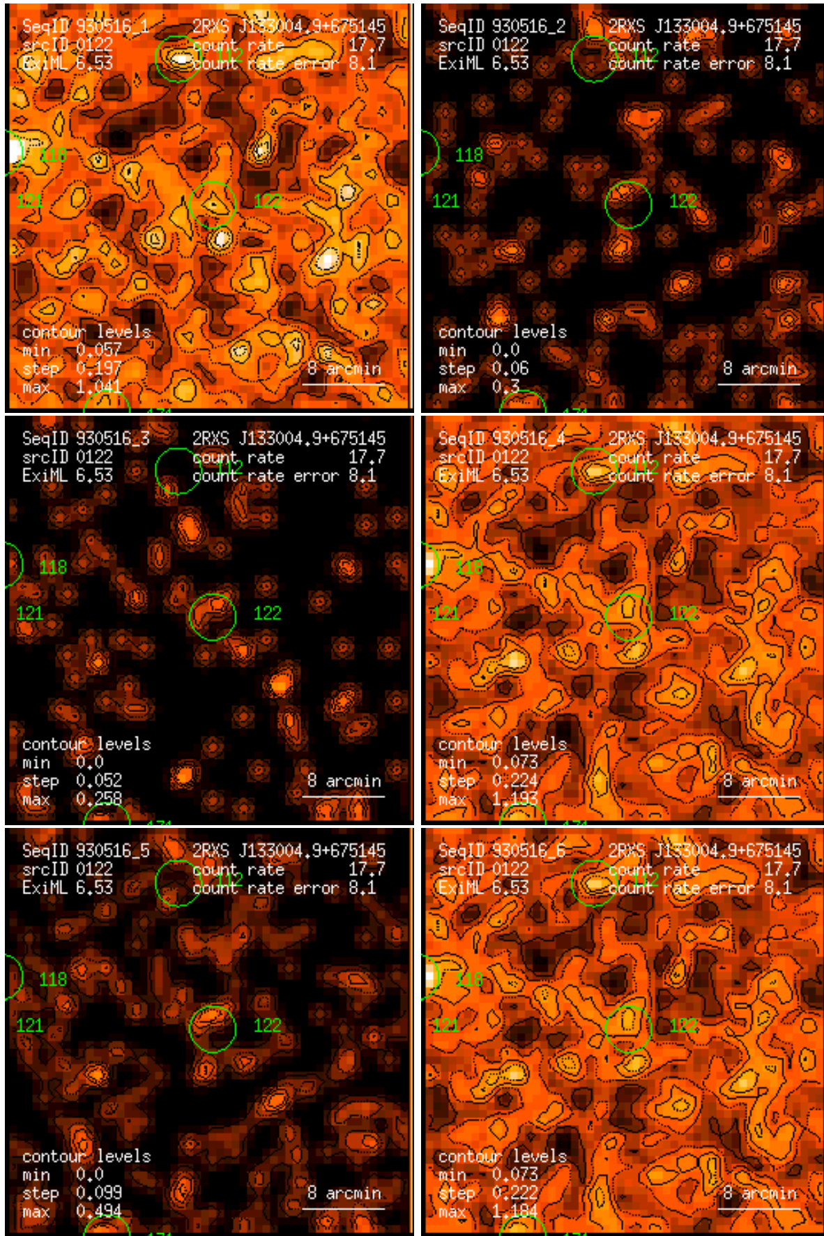
Figure 122: RASS 930516: detection 0122: band rate images, Gaussian filter: (1) PSPC channels 11 – 41, (2) 52 – 90, (3) 91 – 201, (4) 11 – 235, (5) 52 – 201, (6) 11 – 201. Broad band rates in counts/ks. Band rate contour levels in counts/ks/arcmin 2 .
