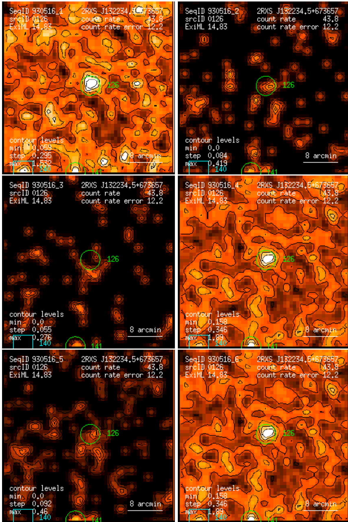
Figure 126: RASS 930516: detection 0126: band rate images, Gaussian filter: (1) PSPC channels 11 – 41, (2) 52 – 90, (3) 91 – 201, (4) 11 – 235, (5) 52 – 201, (6) 11 – 201. Broad band rates in counts/ks. Band rate contour levels in counts/ks/arcmin 2 .
