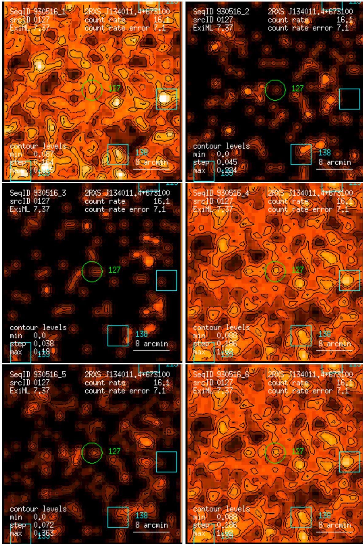
Figure 127: RASS 930516: detection 0127: band rate images, Gaussian filter: (1) PSPC channels 11 – 41, (2) 52 – 90, (3) 91 – 201, (4) 11 – 235, (5) 52 – 201, (6) 11 – 201. Broad band rates in counts/ks. Band rate contour levels in counts/ks/arcmin 2 .
