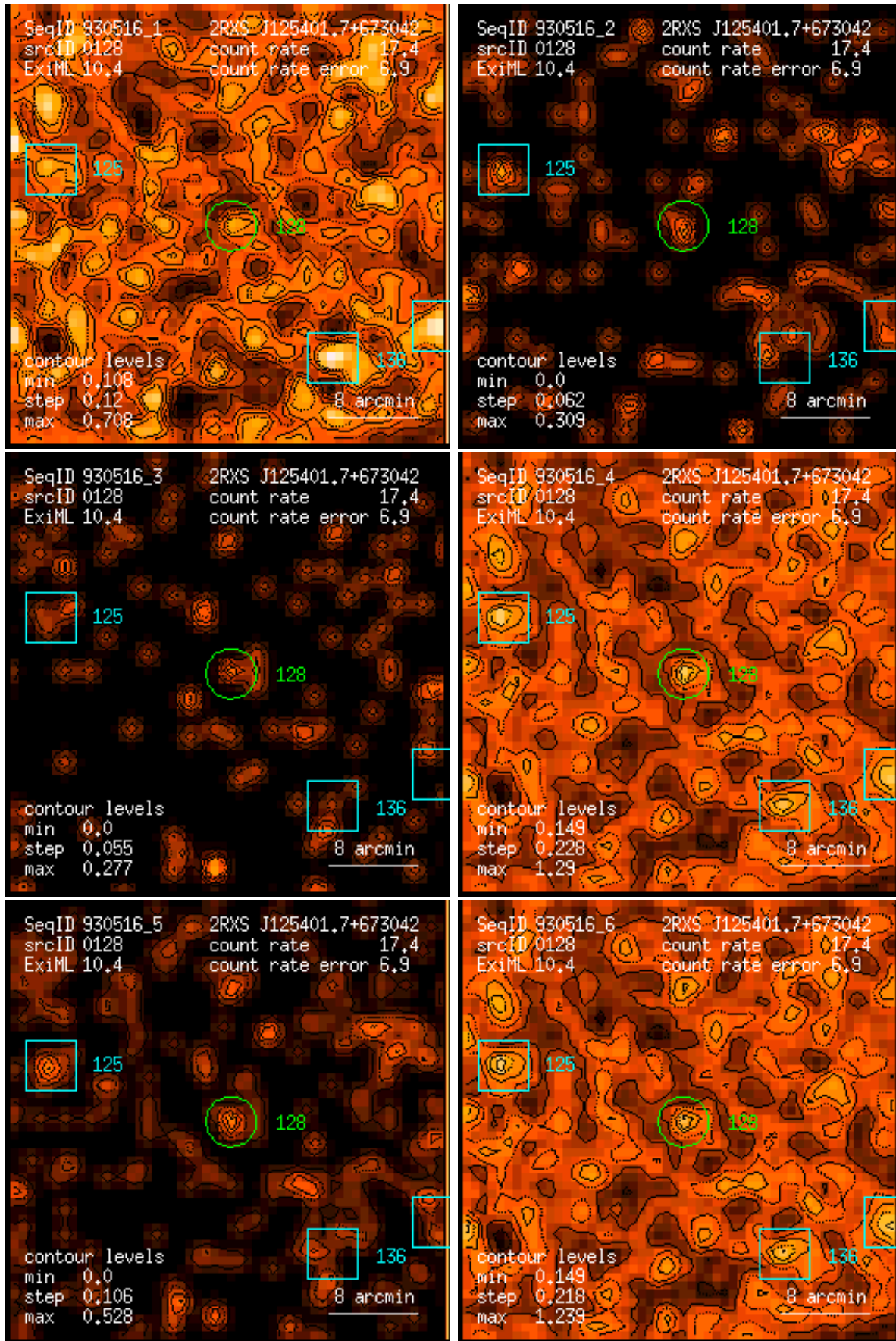
Figure 128: RASS 930516: detection 0128: band rate images, Gaussian filter: (1) PSPC channels 11 – 41, (2) 52 – 90, (3) 91 – 201, (4) 11 – 235, (5) 52 – 201, (6) 11 – 201. Broad band rates in counts/ks. Band rate contour levels in counts/ks/arcmin 2 .
