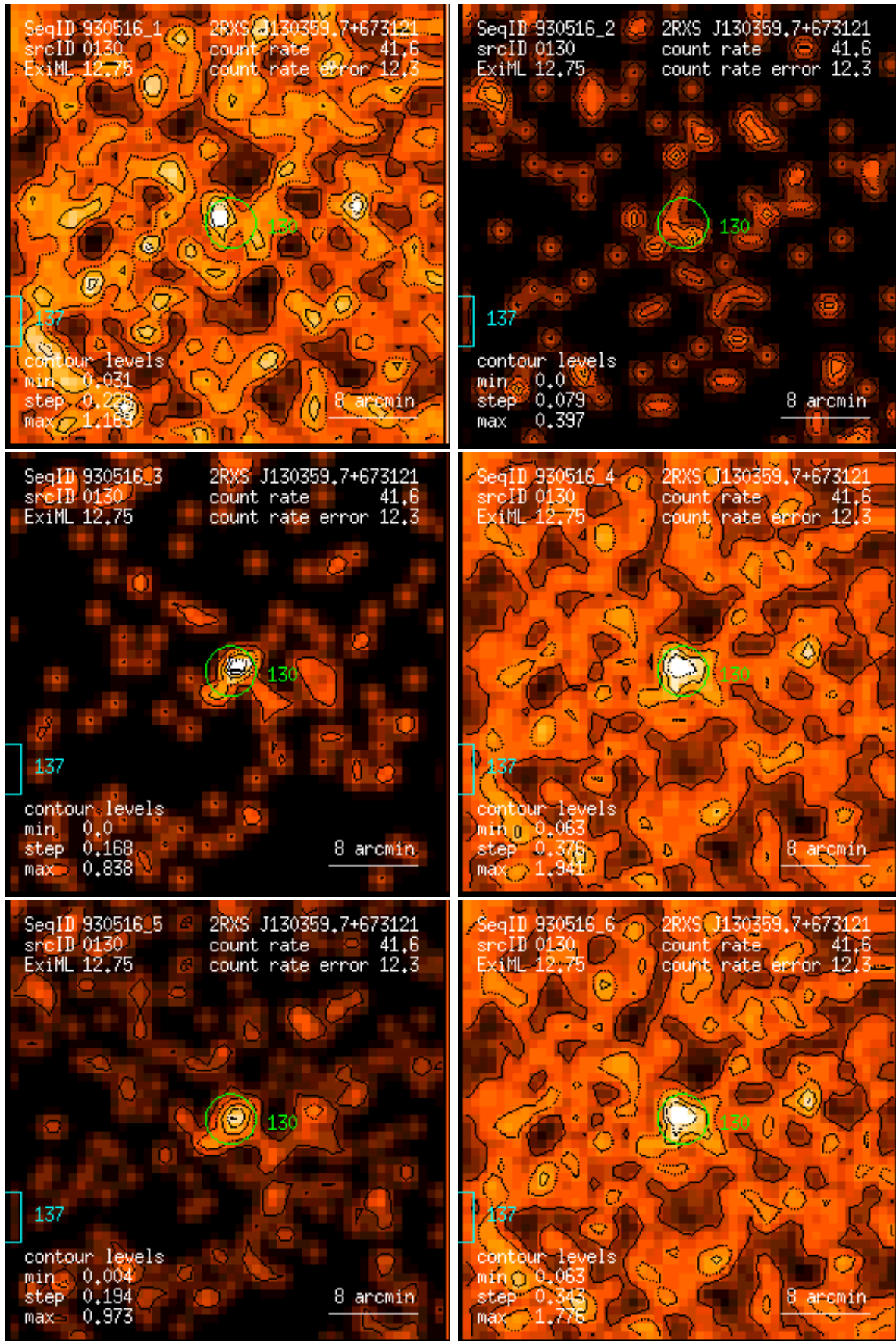
Figure 130: RASS 930516: detection 0130: band rate images, Gaussian filter: (1) PSPC channels 11 – 41, (2) 52 – 90, (3) 91 – 201, (4) 11 – 235, (5) 52 – 201, (6) 11 – 201. Broad band rates in counts/ks. Band rate contour levels in counts/ks/arcmin 2 .
