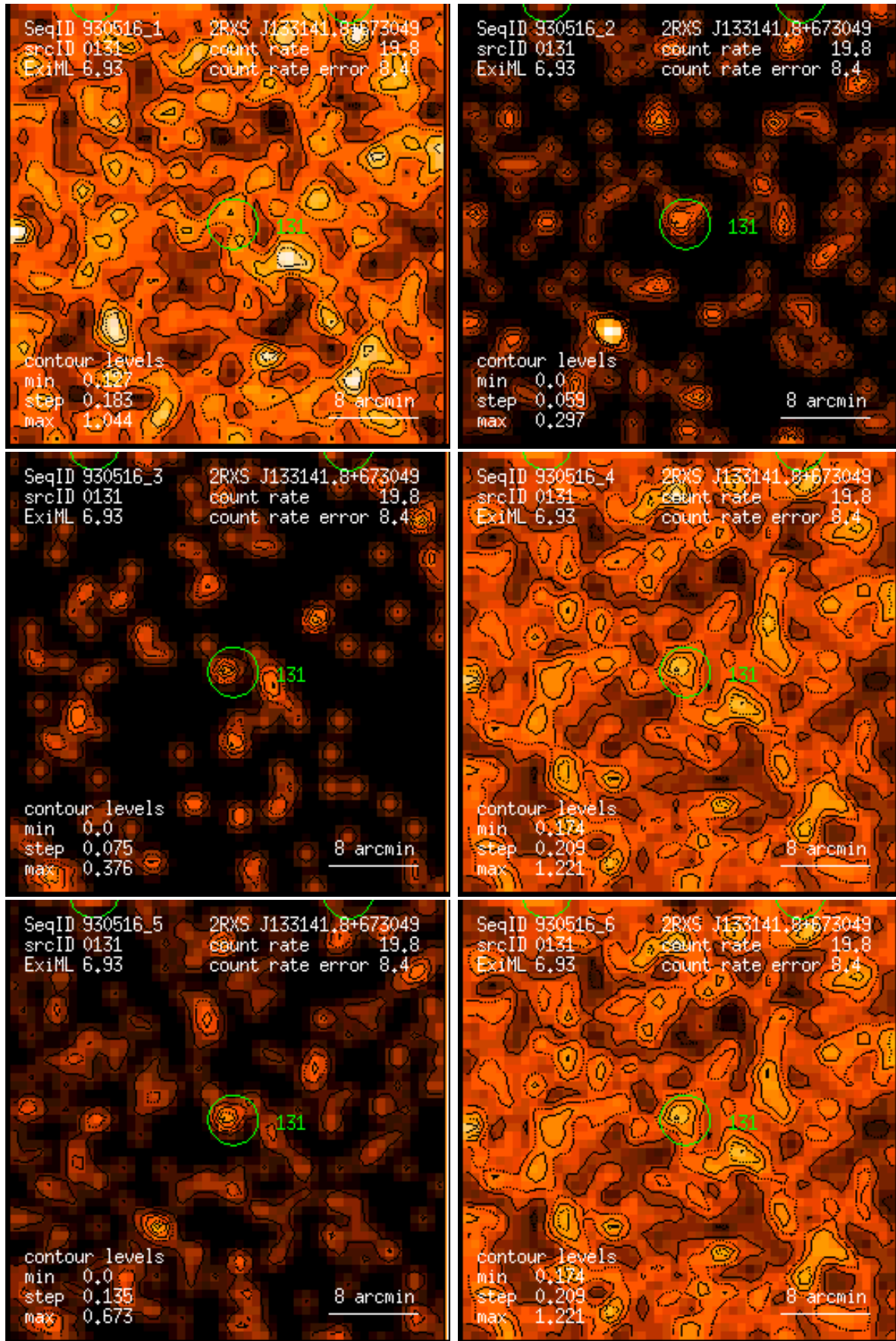
Figure 131: RASS 930516: detection 0131: band rate images, Gaussian filter: (1) PSPC channels 11 – 41, (2) 52 – 90, (3) 91 – 201, (4) 11 – 235, (5) 52 – 201, (6) 11 – 201. Broad band rates in counts/ks. Band rate contour levels in counts/ks/arcmin 2 .
