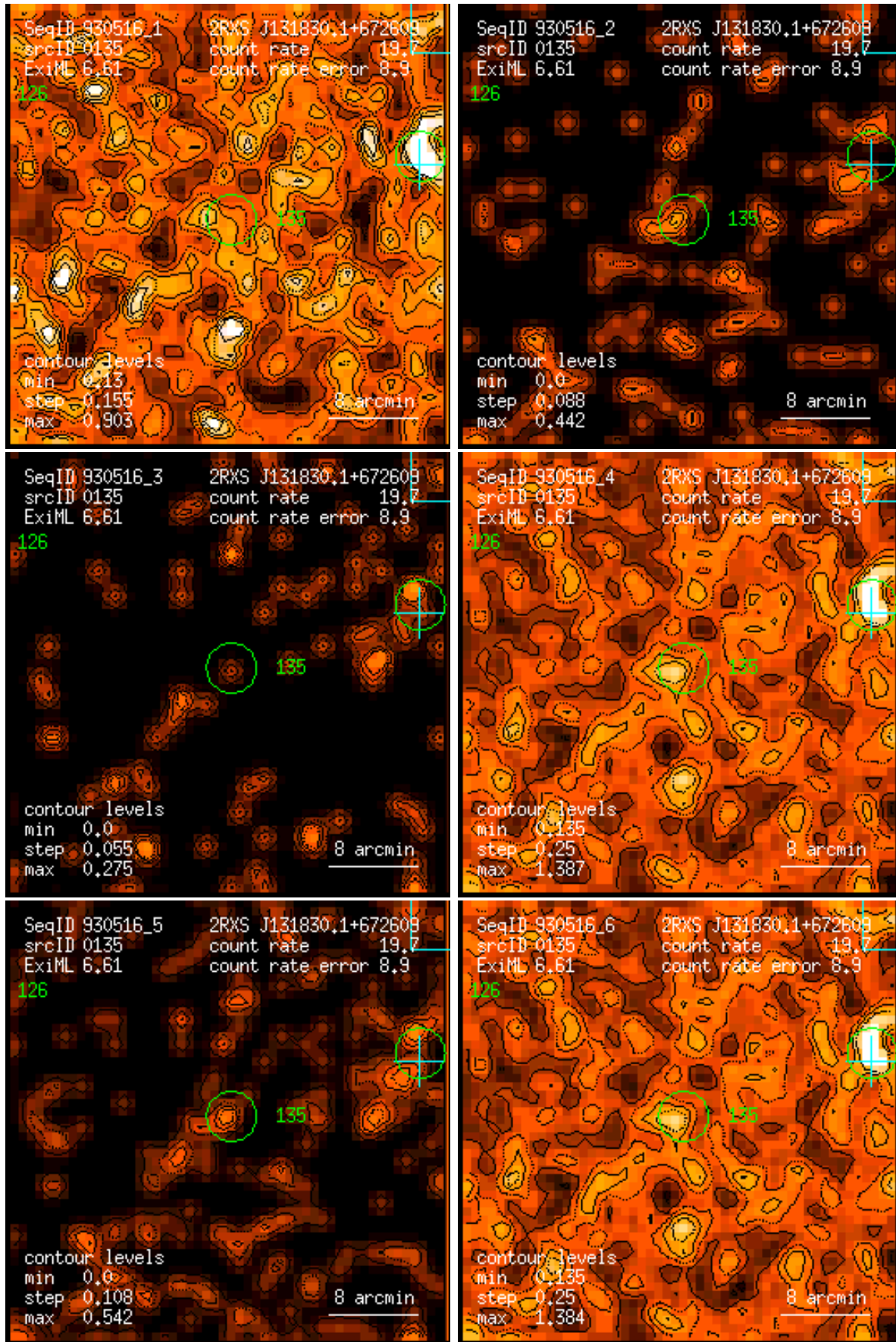
Figure 135: RASS 930516: detection 0135: band rate images, Gaussian filter: (1) PSPC channels 11 – 41, (2) 52 – 90, (3) 91 – 201, (4) 11 – 235, (5) 52 – 201, (6) 11 – 201. Broad band rates in counts/ks. Band rate contour levels in counts/ks/arcmin 2 .
