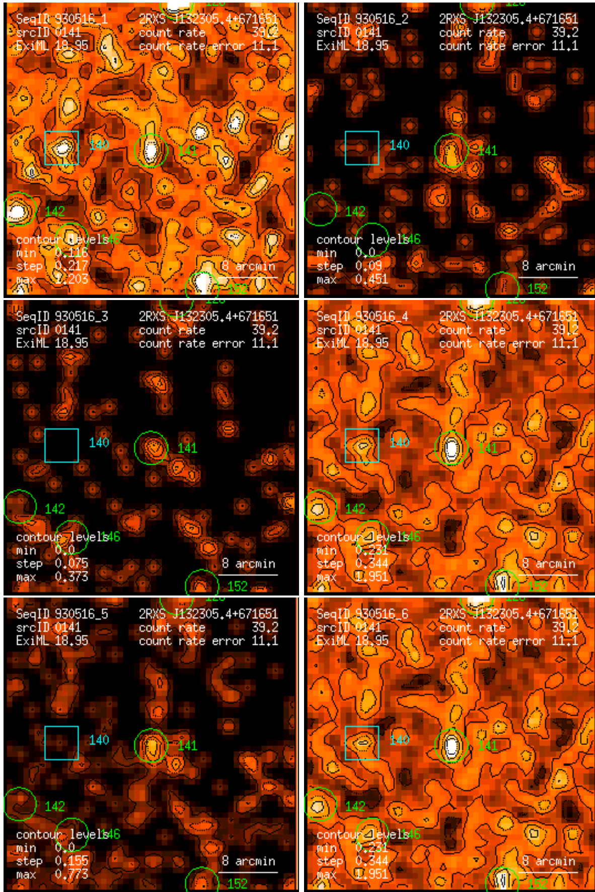
Figure 141: RASS 930516: detection 0141: band rate images, Gaussian filter: (1) PSPC channels 11 – 41, (2) 52 – 90, (3) 91 – 201, (4) 11 – 235, (5) 52 – 201, (6) 11 – 201. Broad band rates in counts/ks. Band rate contour levels in counts/ks/arcmin 2 .
