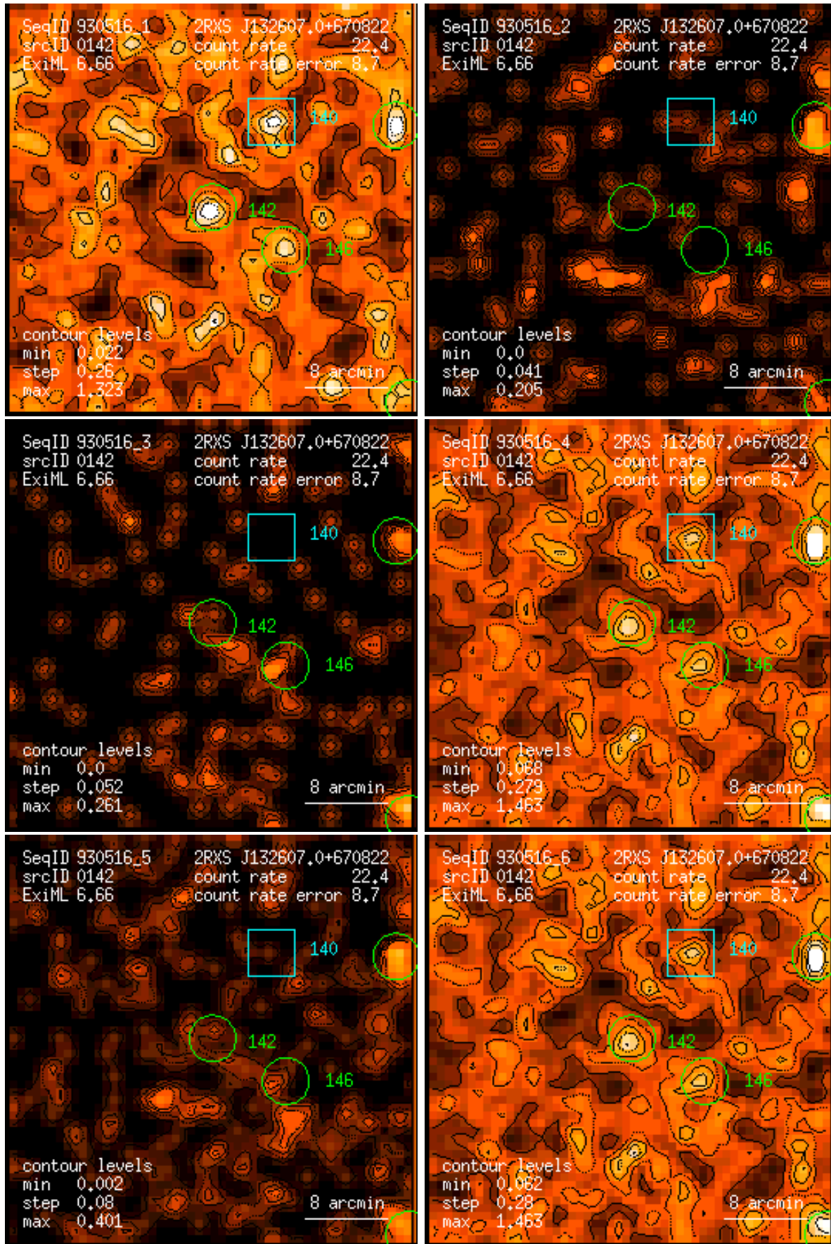
Figure 142: RASS 930516: detection 0142: band rate images, Gaussian filter: (1) PSPC channels 11 – 41, (2) 52 – 90, (3) 91 – 201, (4) 11 – 235, (5) 52 – 201, (6) 11 – 201. Broad band rates in counts/ks. Band rate contour levels in counts/ks/arcmin 2 .
