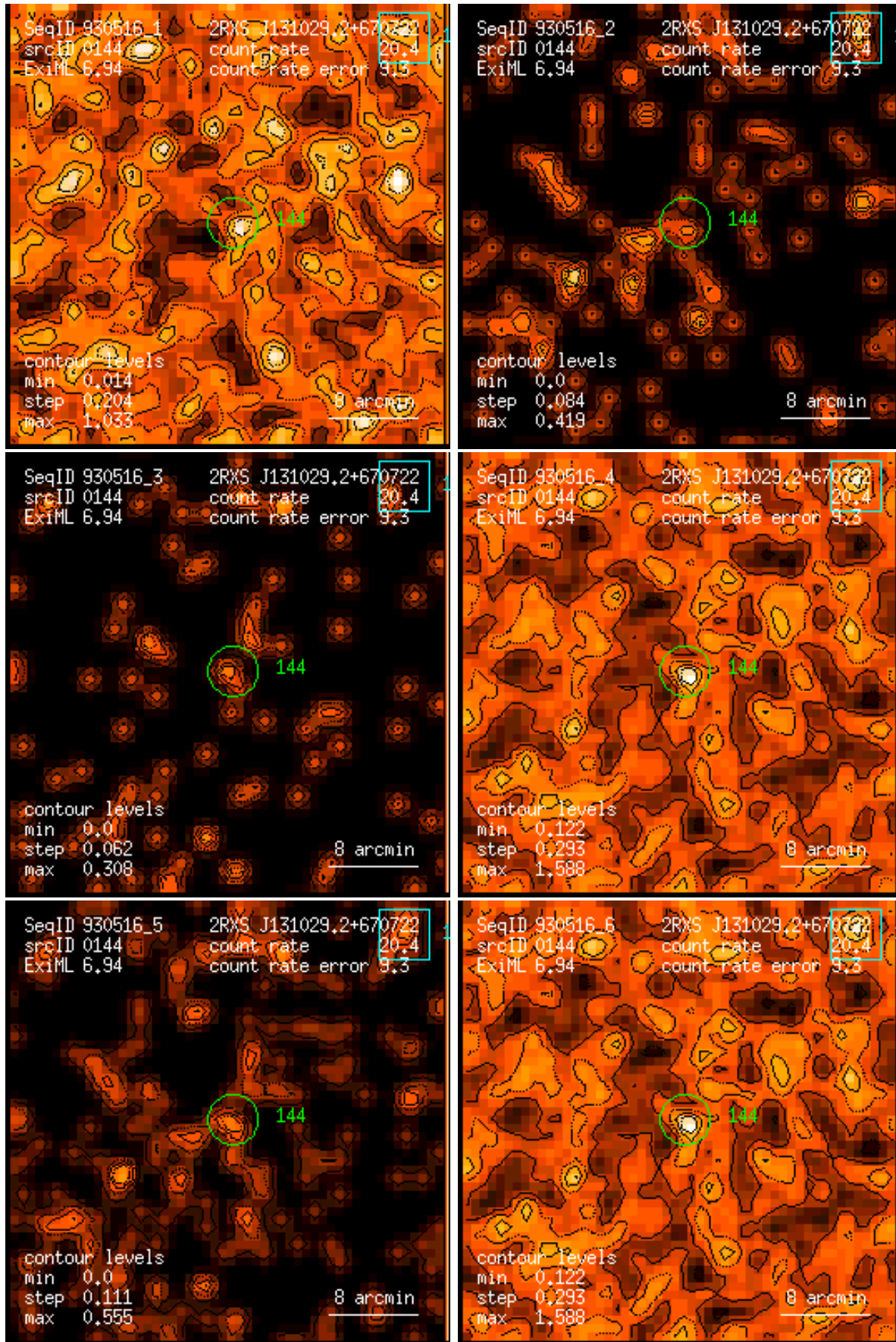
Figure 144: RASS 930516: detection 0144: band rate images, Gaussian filter: (1) PSPC channels 11 – 41, (2) 52 – 90, (3) 91 – 201, (4) 11 – 235, (5) 52 – 201, (6) 11 – 201. Broad band rates in counts/ks. Band rate contour levels in counts/ks/arcmin 2 .
