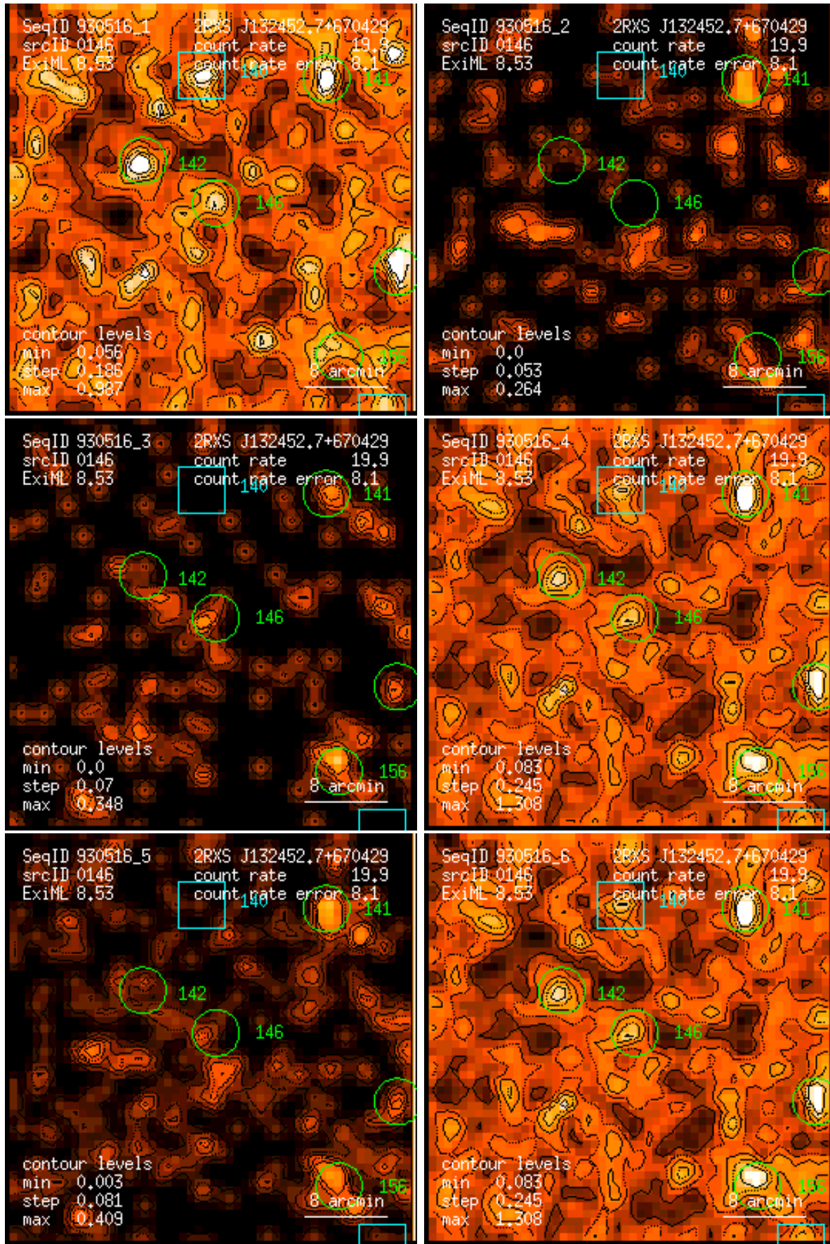
Figure 146: RASS 930516: detection 0146: band rate images, Gaussian filter: (1) PSPC channels 11 – 41, (2) 52 – 90, (3) 91 – 201, (4) 11 – 235, (5) 52 – 201, (6) 11 – 201. Broad band rates in counts/ks. Band rate contour levels in counts/ks/arcmin 2 .
