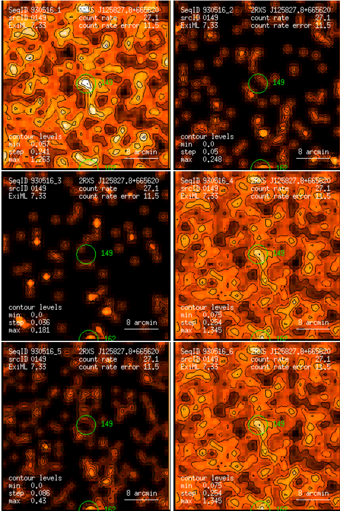
Figure 149: RASS 930516: detection 0149: band rate images, Gaussian filter: (1) PSPC channels 11 – 41, (2) 52 – 90, (3) 91 – 201, (4) 11 – 235, (5) 52 – 201, (6) 11 – 201. Broad band rates in counts/ks. Band rate contour levels in counts/ks/arcmin 2 .
