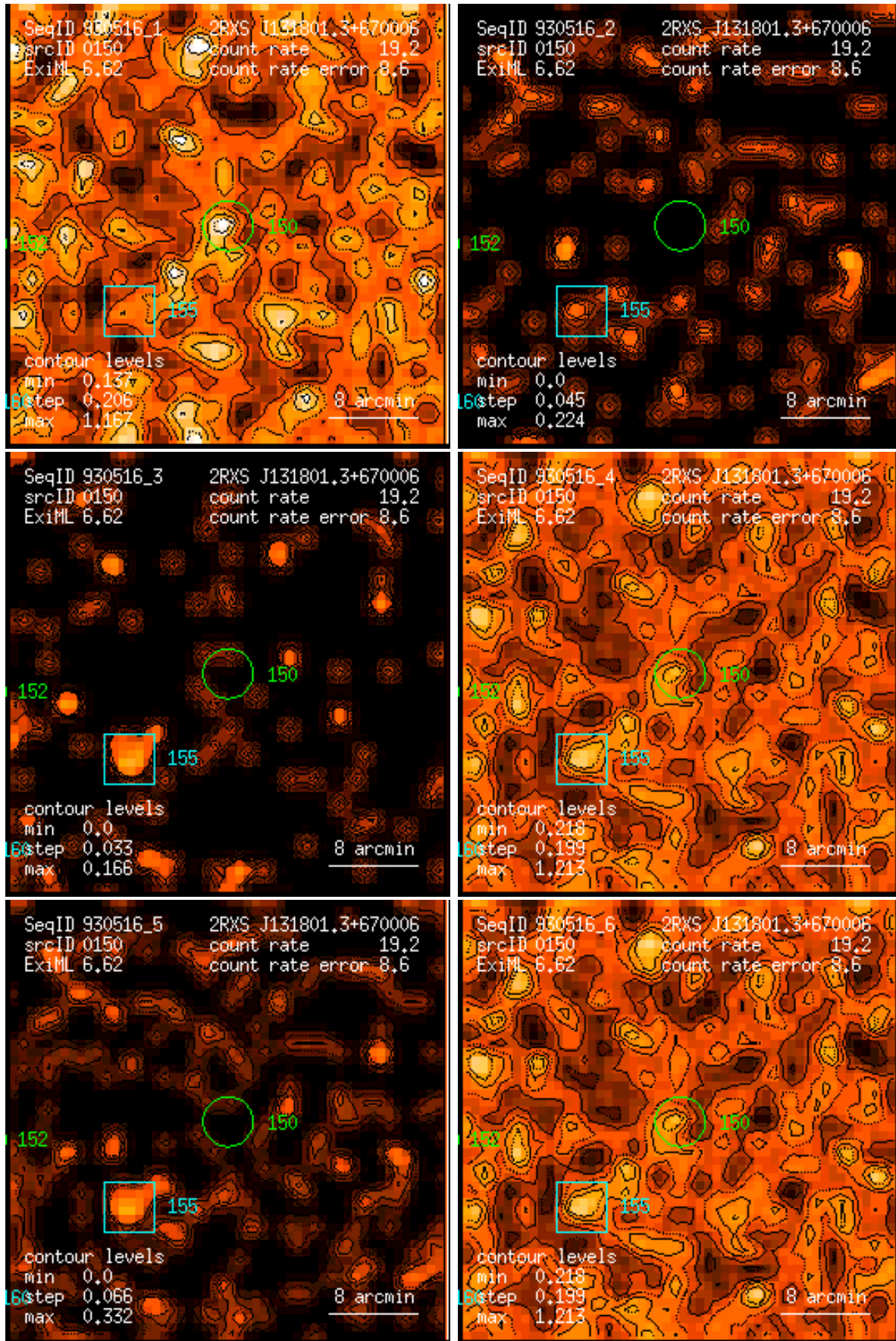
Figure 150: RASS 930516: detection 0150: band rate images, Gaussian filter: (1) PSPC channels 11 – 41, (2) 52 – 90, (3) 91 – 201, (4) 11 – 235, (5) 52 – 201, (6) 11 – 201. Broad band rates in counts/ks. Band rate contour levels in counts/ks/arcmin 2 .
