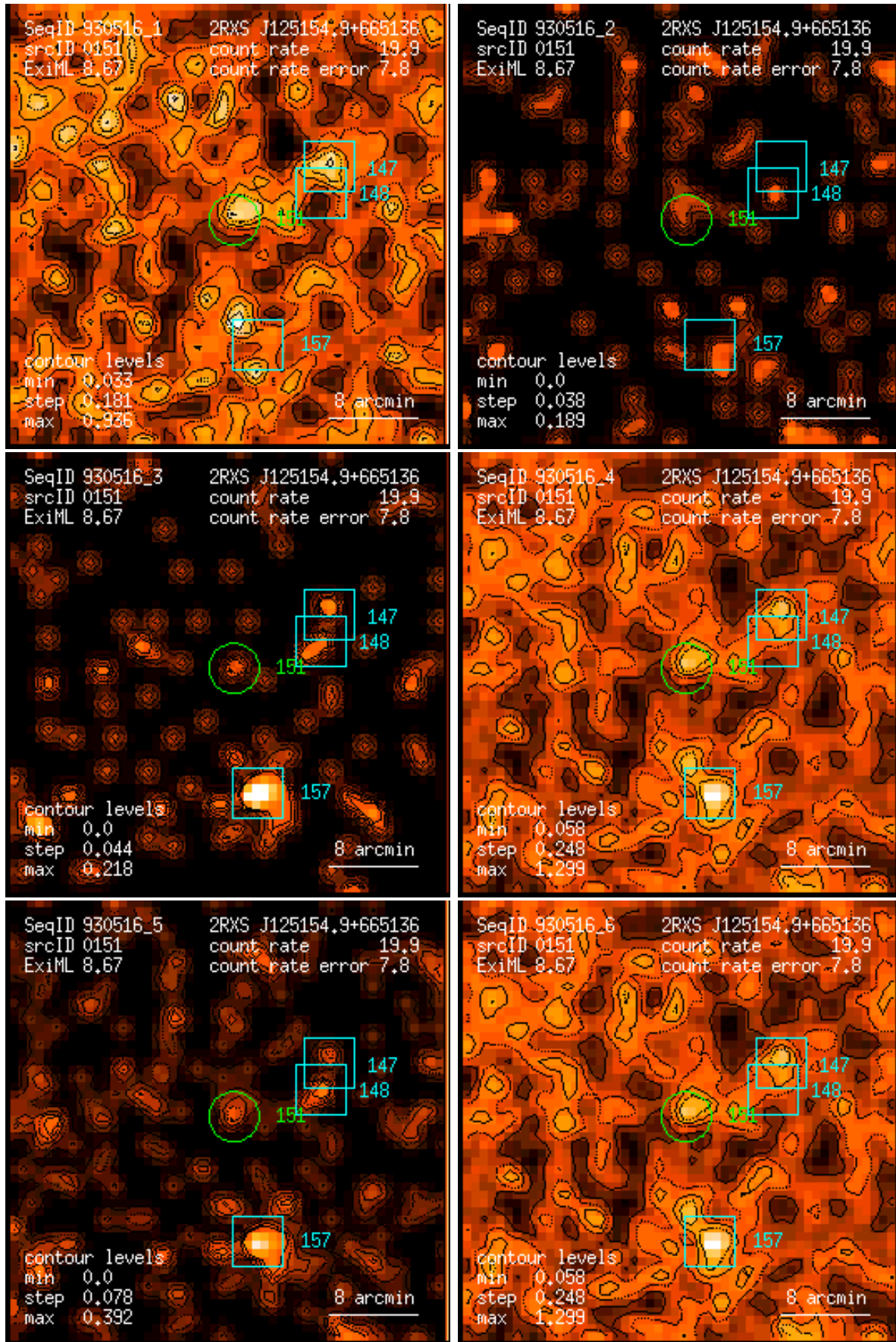
Figure 151: RASS 930516: detection 0151: band rate images, Gaussian filter: (1) PSPC channels 11 – 41, (2) 52 – 90, (3) 91 – 201, (4) 11 – 235, (5) 52 – 201, (6) 11 – 201. Broad band rates in counts/ks. Band rate contour levels in counts/ks/arcmin 2 .
