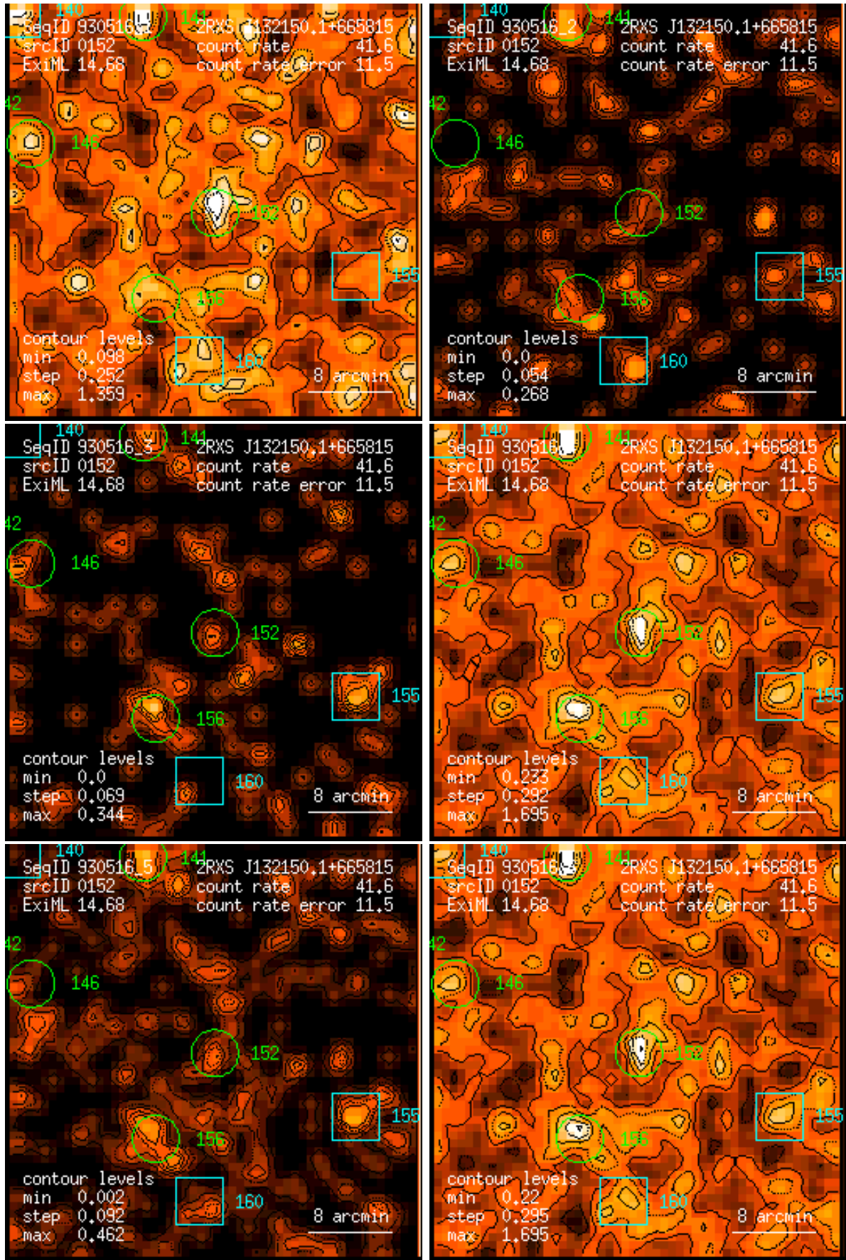
Figure 152: RASS 930516: detection 0152: band rate images, Gaussian filter: (1) PSPC channels 11 – 41, (2) 52 – 90, (3) 91 – 201, (4) 11 – 235, (5) 52 – 201, (6) 11 – 201. Broad band rates in counts/ks. Band rate contour levels in counts/ks/arcmin 2 .
