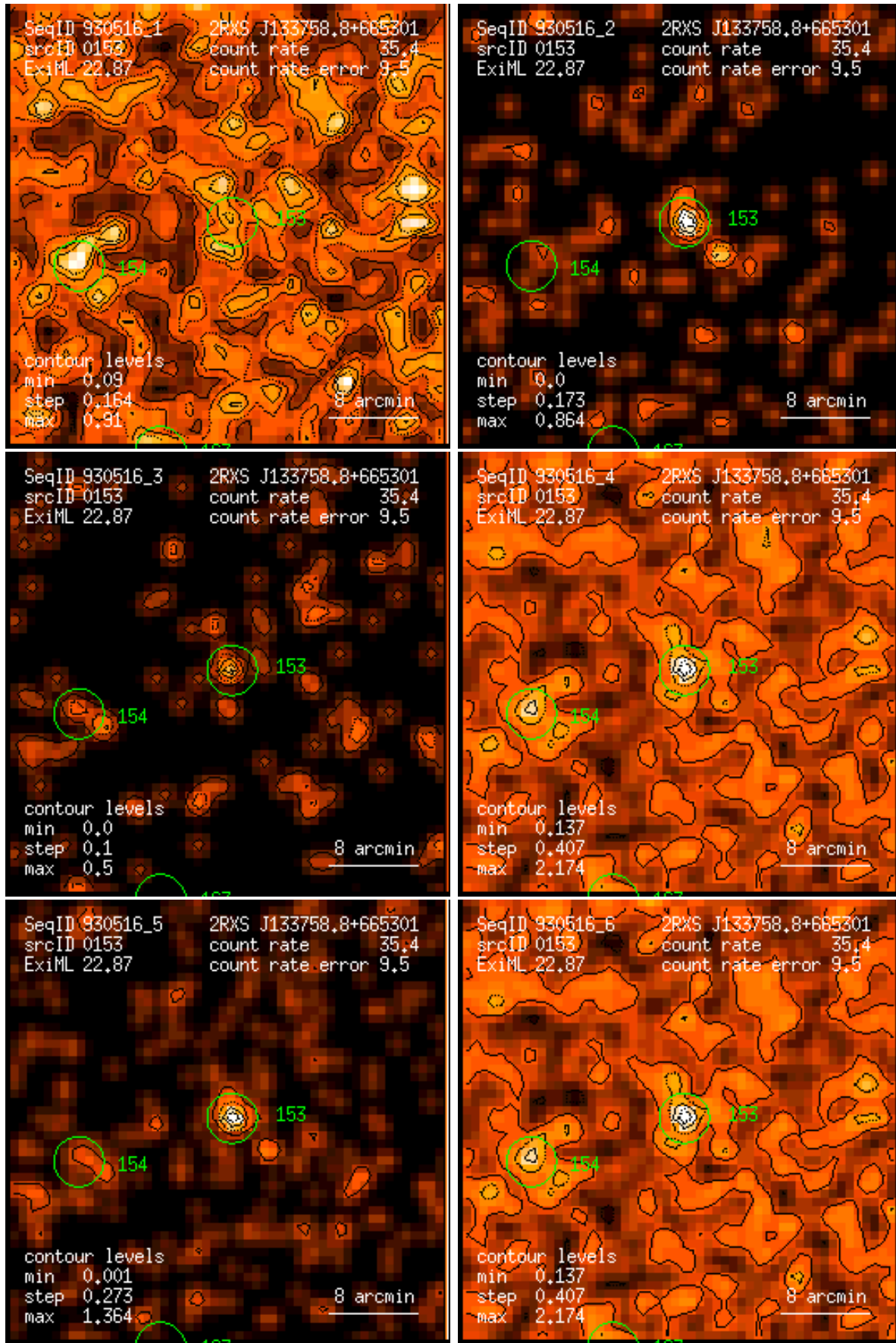
Figure 153: RASS 930516: detection 0153: band rate images, Gaussian filter: (1) PSPC channels 11 – 41, (2) 52 – 90, (3) 91 – 201, (4) 11 – 235, (5) 52 – 201, (6) 11 – 201. Broad band rates in counts/ks. Band rate contour levels in counts/ks/arcmin 2 .
