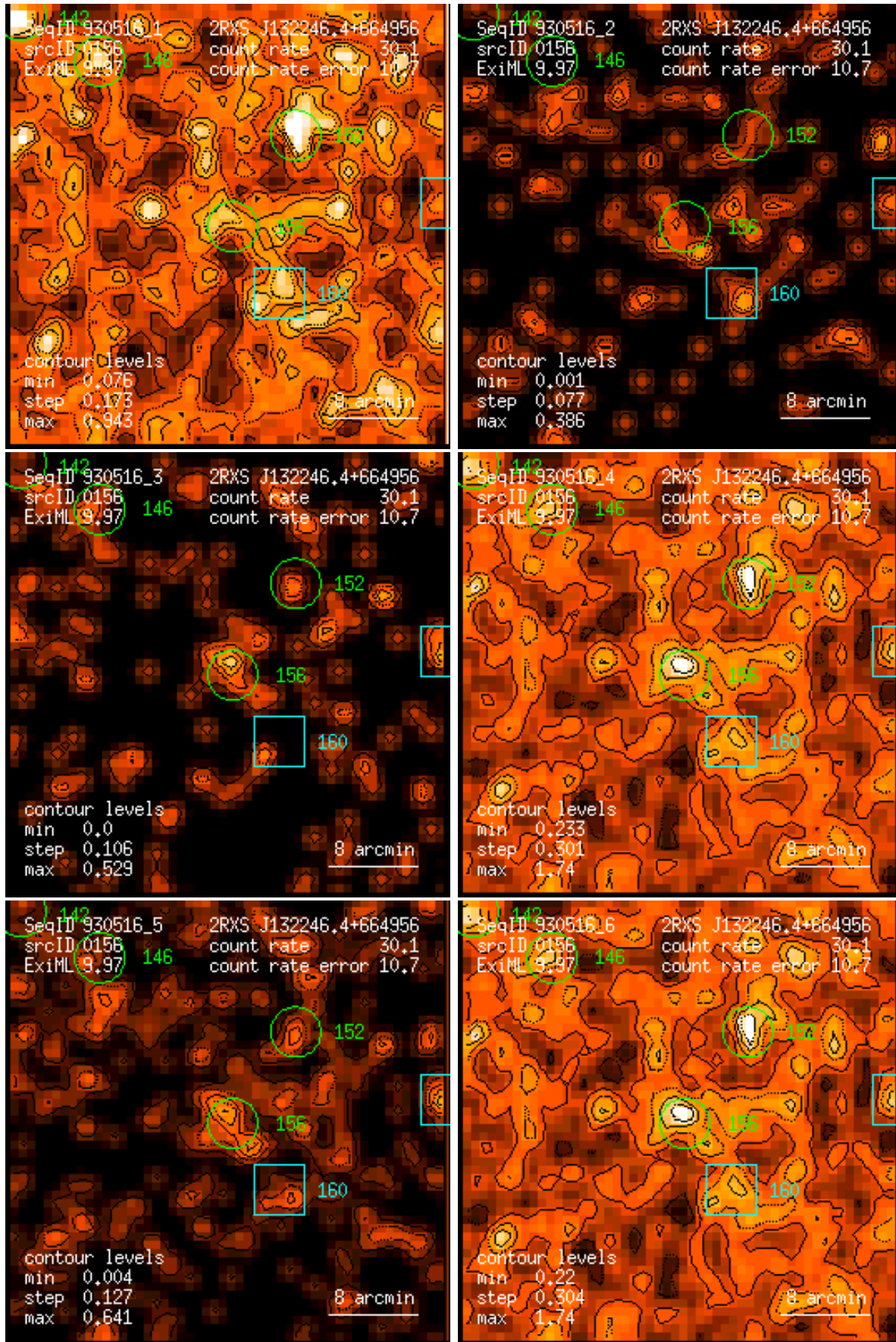
Figure 156: RASS 930516: detection 0156: band rate images, Gaussian filter: (1) PSPC channels 11 – 41, (2) 52 – 90, (3) 91 – 201, (4) 11 – 235, (5) 52 – 201, (6) 11 – 201. Broad band rates in counts/ks. Band rate contour levels in counts/ks/arcmin 2 .
