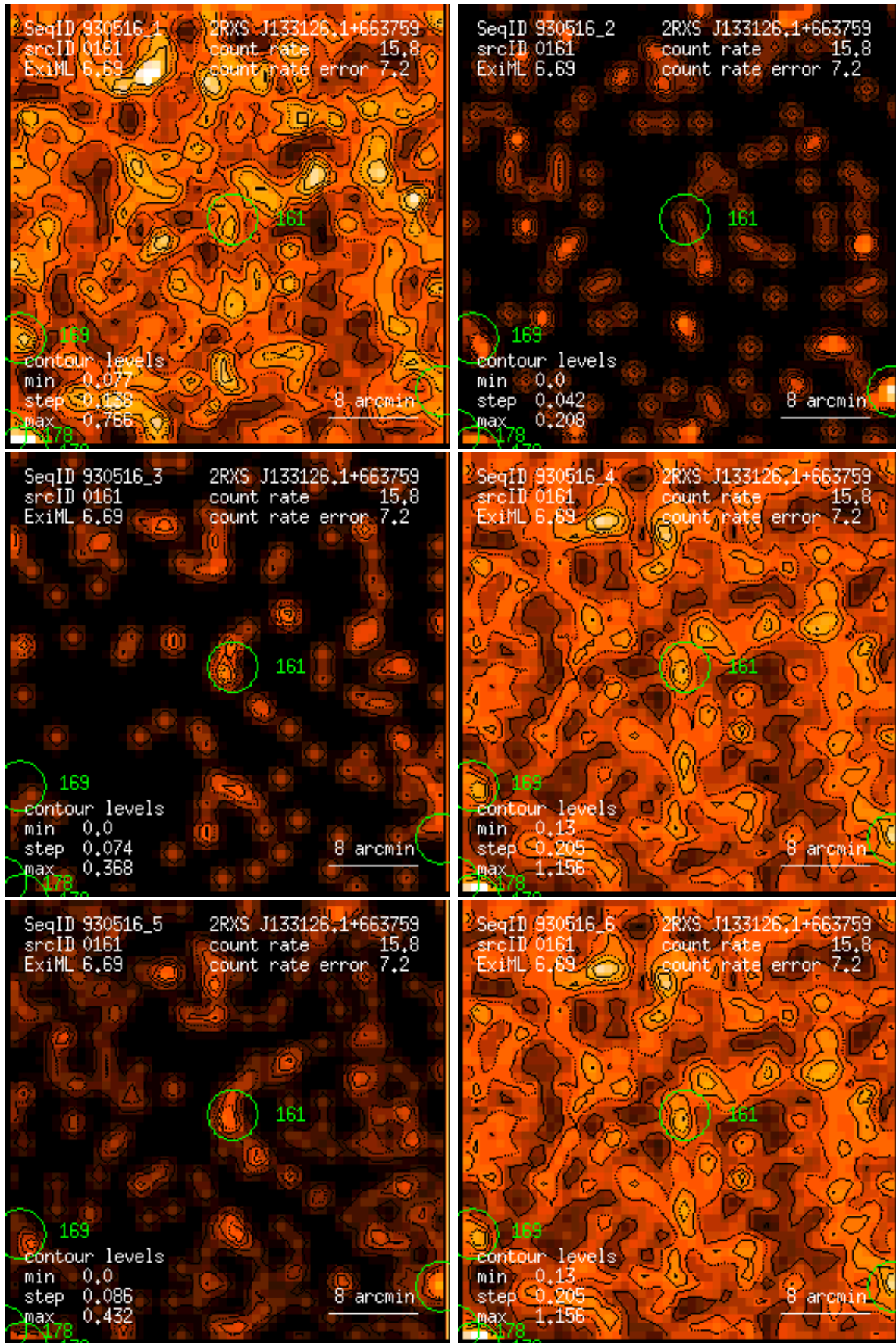
Figure 161: RASS 930516: detection 0161: band rate images, Gaussian filter: (1) PSPC channels 11 – 41, (2) 52 – 90, (3) 91 – 201, (4) 11 – 235, (5) 52 – 201, (6) 11 – 201. Broad band rates in counts/ks. Band rate contour levels in counts/ks/arcmin 2 .
