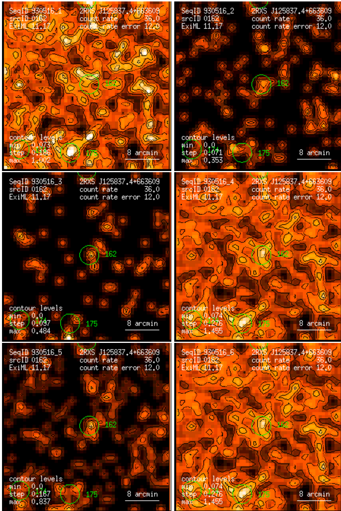
Figure 162: RASS 930516: detection 0162: band rate images, Gaussian filter: (1) PSPC channels 11 – 41, (2) 52 – 90, (3) 91 – 201, (4) 11 – 235, (5) 52 – 201, (6) 11 – 201. Broad band rates in counts/ks. Band rate contour levels in counts/ks/arcmin 2 .
