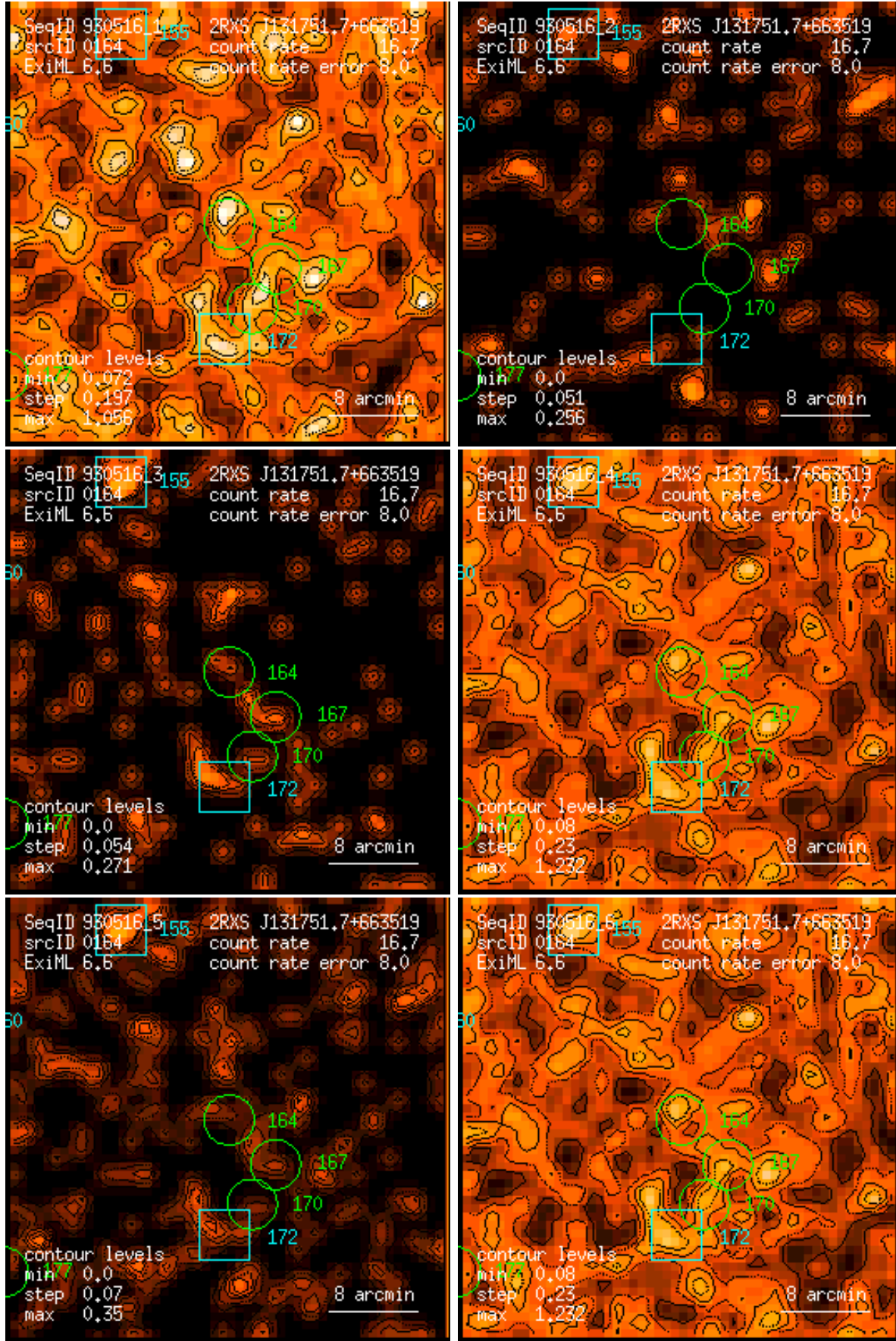
Figure 164: RASS 930516: detection 0164: band rate images, Gaussian filter: (1) PSPC channels 11 – 41, (2) 52 – 90, (3) 91 – 201, (4) 11 – 235, (5) 52 – 201, (6) 11 – 201. Broad band rates in counts/ks. Band rate contour levels in counts/ks/arcmin 2 .
