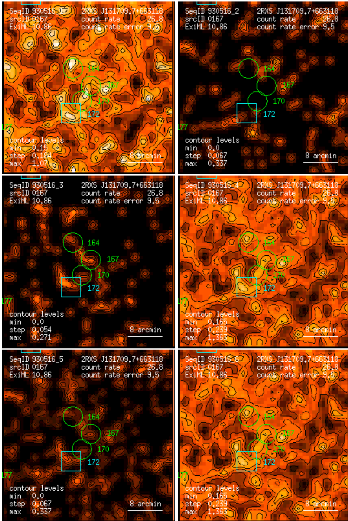
Figure 167: RASS 930516: detection 0167: band rate images, Gaussian filter: (1) PSPC channels 11 – 41, (2) 52 – 90, (3) 91 – 201, (4) 11 – 235, (5) 52 – 201, (6) 11 – 201. Broad band rates in counts/ks. Band rate contour levels in counts/ks/arcmin 2 .
