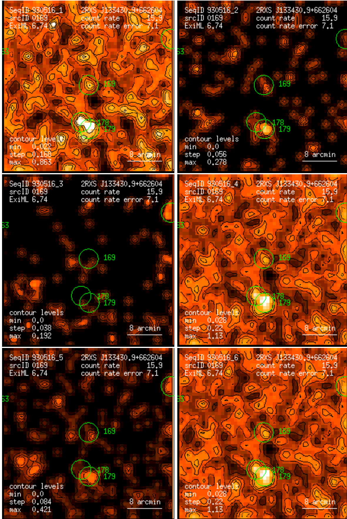
Figure 169: RASS 930516: detection 0169: band rate images, Gaussian filter: (1) PSPC channels 11 – 41, (2) 52 – 90, (3) 91 – 201, (4) 11 – 235, (5) 52 – 201, (6) 11 – 201. Broad band rates in counts/ks. Band rate contour levels in counts/ks/arcmin 2 .
