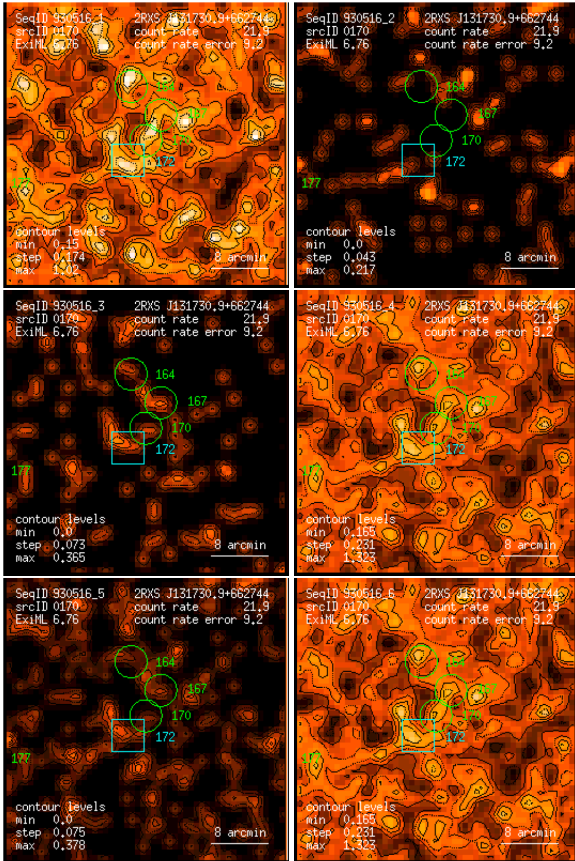
Figure 170: RASS 930516: detection 0170: band rate images, Gaussian filter: (1) PSPC channels 11 – 41, (2) 52 – 90, (3) 91 – 201, (4) 11 – 235, (5) 52 – 201, (6) 11 – 201. Broad band rates in counts/ks. Band rate contour levels in counts/ks/arcmin 2 .
