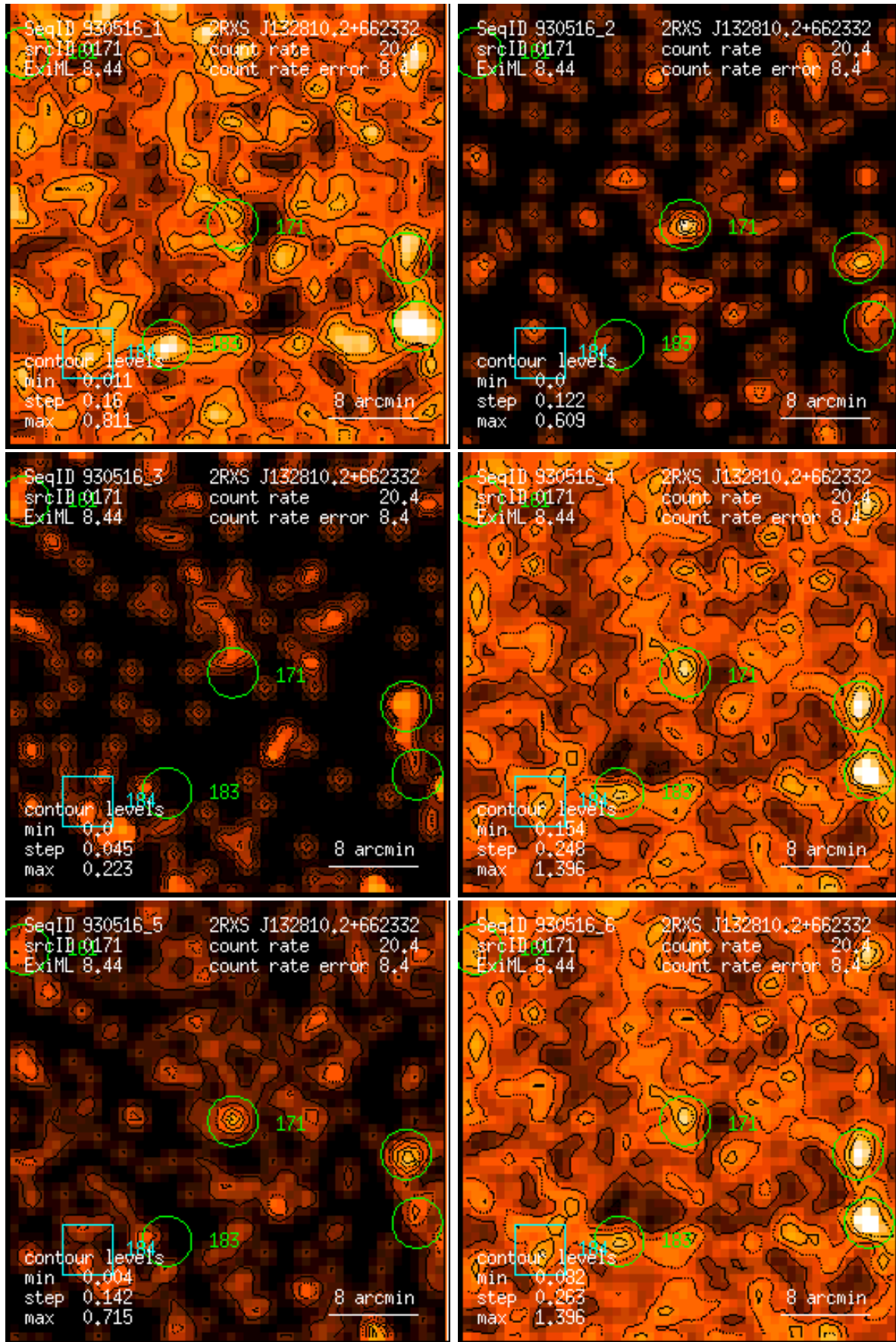
Figure 171: RASS 930516: detection 0171: band rate images, Gaussian filter: (1) PSPC channels 11 – 41, (2) 52 – 90, (3) 91 – 201, (4) 11 – 235, (5) 52 – 201, (6) 11 – 201. Broad band rates in counts/ks. Band rate contour levels in counts/ks/arcmin 2 .
