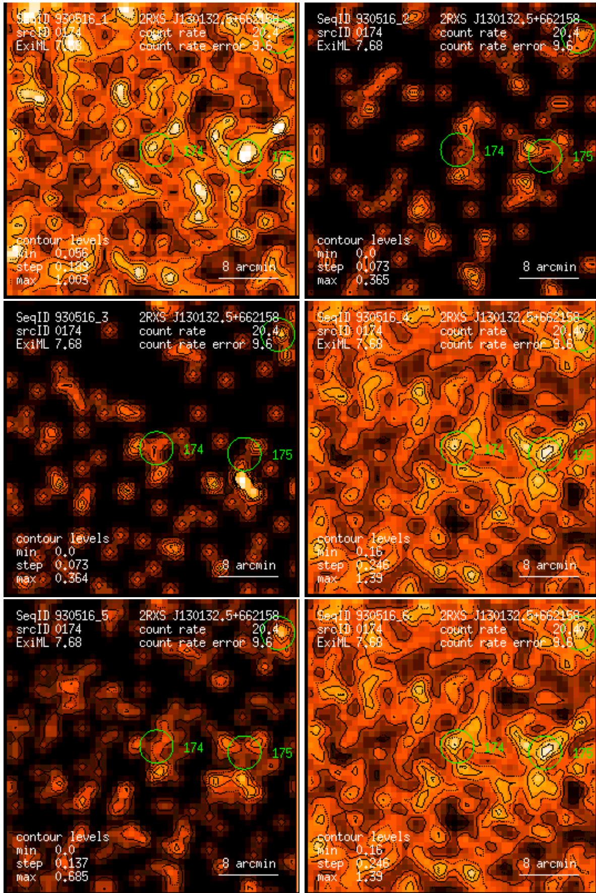
Figure 174: RASS 930516: detection 0174: band rate images, Gaussian filter: (1) PSPC channels 11 – 41, (2) 52 – 90, (3) 91 – 201, (4) 11 – 235, (5) 52 – 201, (6) 11 – 201. Broad band rates in counts/ks. Band rate contour levels in counts/ks/arcmin 2 .
