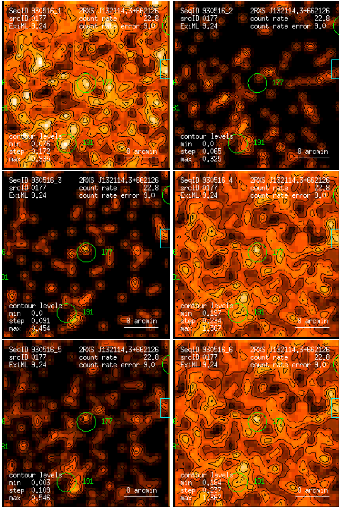
Figure 177: RASS 930516: detection 0177: band rate images, Gaussian filter: (1) PSPC channels 11 – 41, (2) 52 – 90, (3) 91 – 201, (4) 11 – 235, (5) 52 – 201, (6) 11 – 201. Broad band rates in counts/ks. Band rate contour levels in counts/ks/arcmin 2 .
