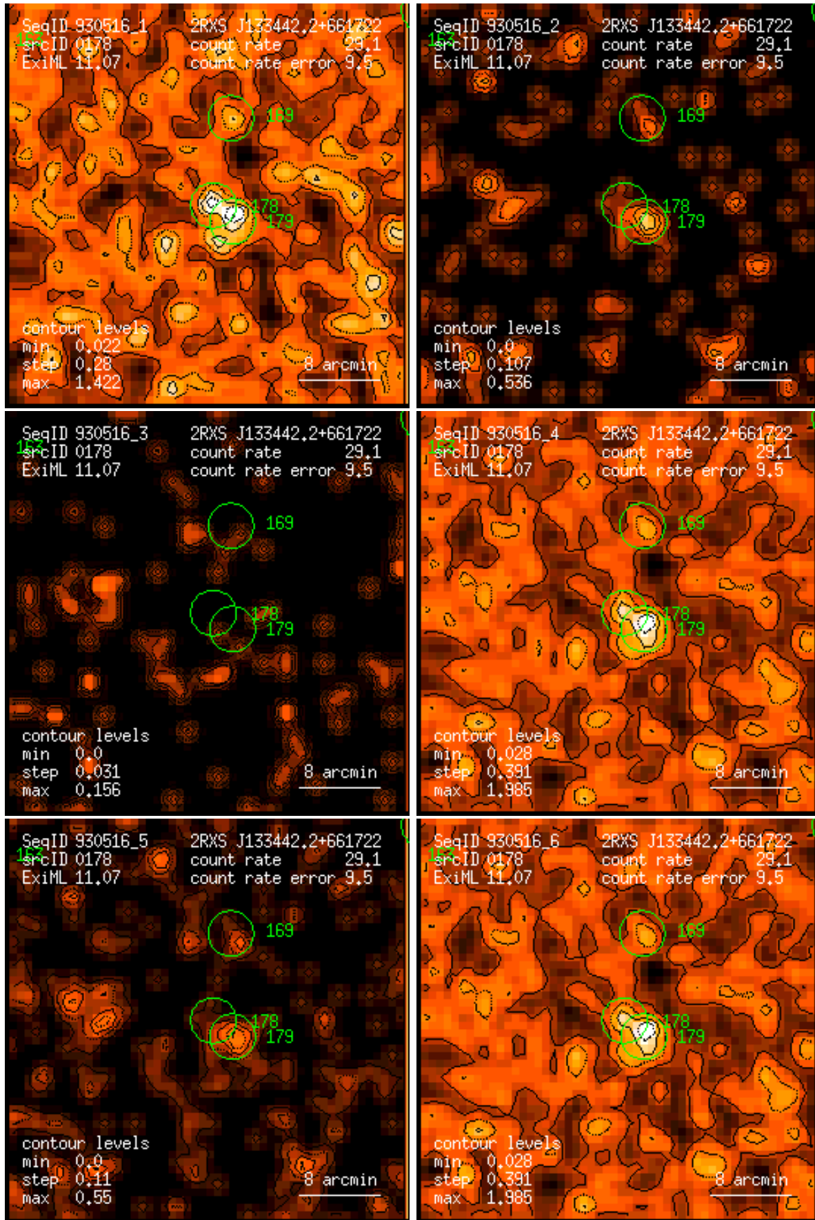
Figure 178: RASS 930516: detection 0178: band rate images, Gaussian filter: (1) PSPC channels 11 – 41, (2) 52 – 90, (3) 91 – 201, (4) 11 – 235, (5) 52 – 201, (6) 11 – 201. Broad band rates in counts/ks. Band rate contour levels in counts/ks/arcmin 2 .
