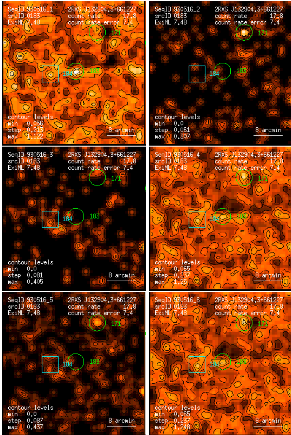
Figure 183: RASS 930516: detection 0183: band rate images, Gaussian filter: (1) PSPC channels 11 – 41, (2) 52 – 90, (3) 91 – 201, (4) 11 – 235, (5) 52 – 201, (6) 11 – 201. Broad band rates in counts/ks. Band rate contour levels in counts/ks/arcmin 2 .
