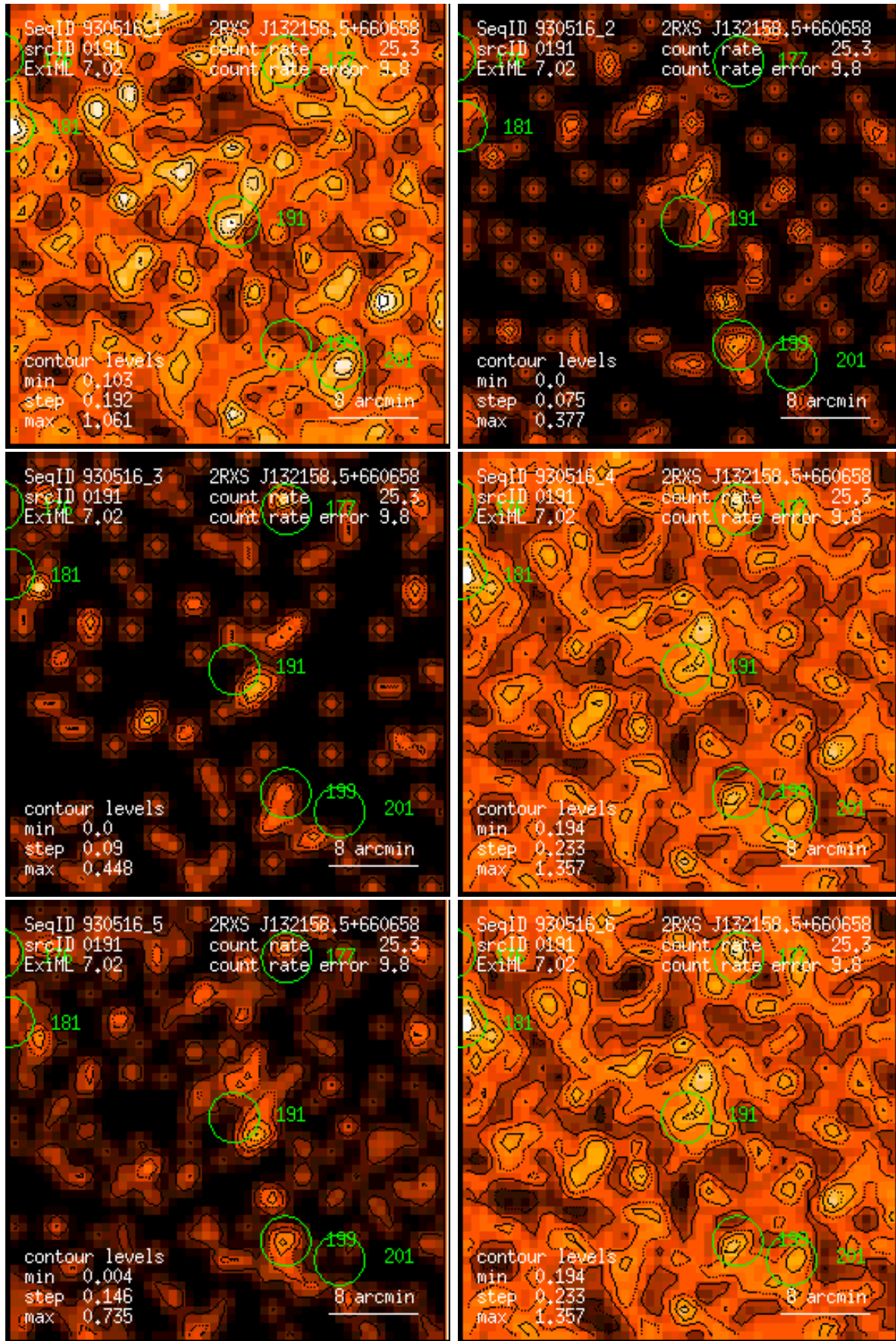
Figure 191: RASS 930516: detection 0191: band rate images, Gaussian filter: (1) PSPC channels 11 – 41, (2) 52 – 90, (3) 91 – 201, (4) 11 – 235, (5) 52 – 201, (6) 11 – 201. Broad band rates in counts/ks. Band rate contour levels in counts/ks/arcmin 2 .
