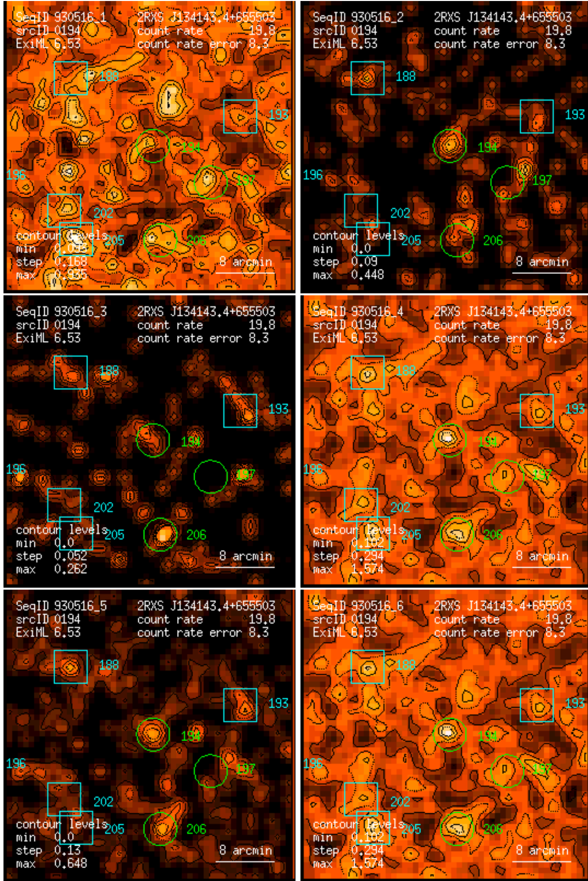
Figure 194: RASS 930516: detection 0194: band rate images, Gaussian filter: (1) PSPC channels 11 – 41, (2) 52 – 90, (3) 91 – 201, (4) 11 – 235, (5) 52 – 201, (6) 11 – 201. Broad band rates in counts/ks. Band rate contour levels in counts/ks/arcmin 2 .
