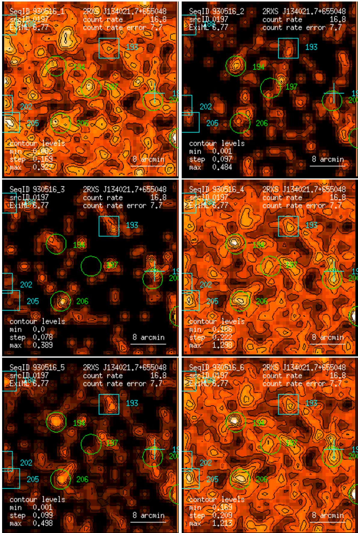
Figure 197: RASS 930516: detection 0197: band rate images, Gaussian filter: (1) PSPC channels 11 – 41, (2) 52 – 90, (3) 91 – 201, (4) 11 – 235, (5) 52 – 201, (6) 11 – 201. Broad band rates in counts/ks. Band rate contour levels in counts/ks/arcmin 2 .
