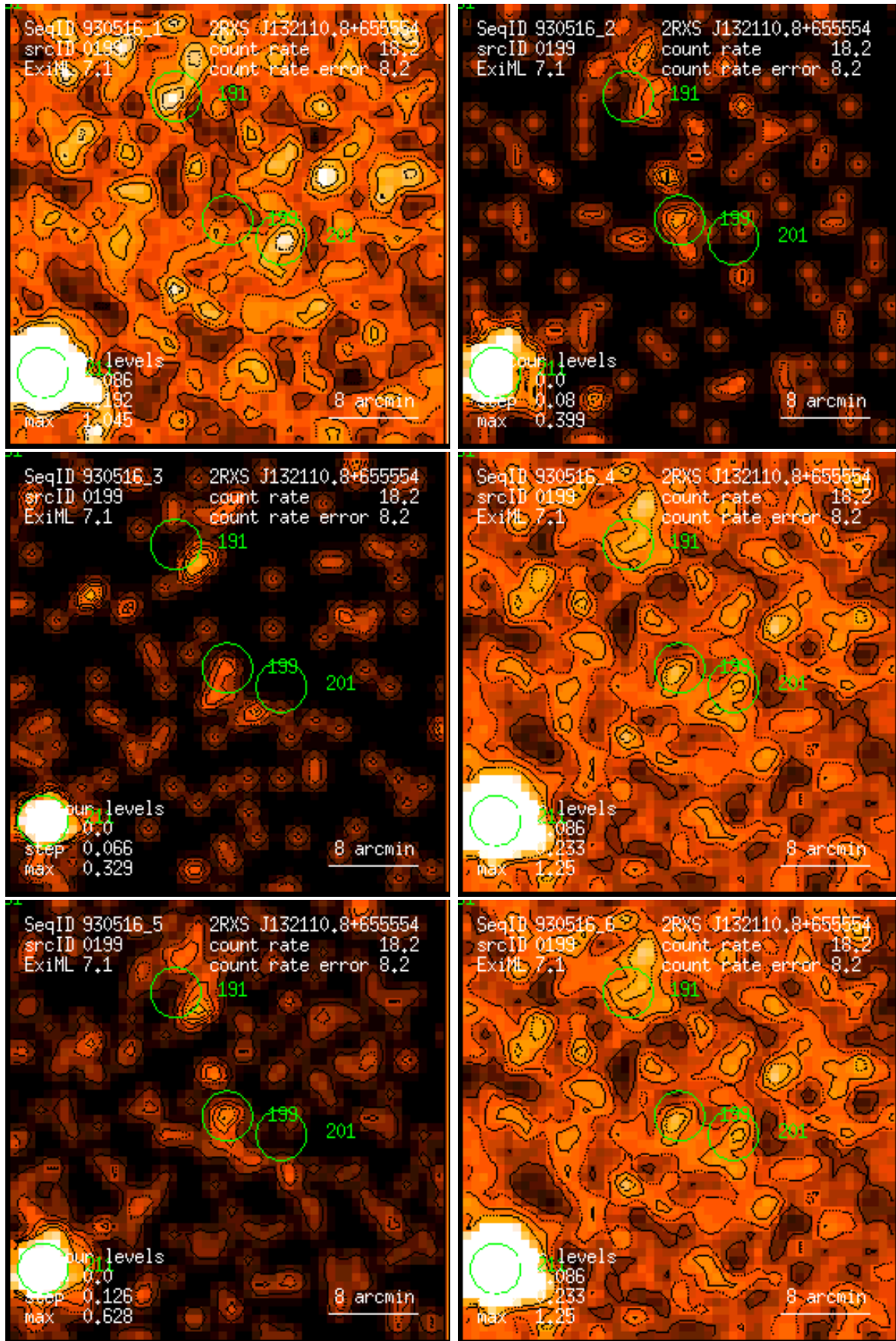
Figure 199: RASS 930516: detection 0199: band rate images, Gaussian filter: (1) PSPC channels 11 – 41, (2) 52 – 90, (3) 91 – 201, (4) 11 – 235, (5) 52 – 201, (6) 11 – 201. Broad band rates in counts/ks. Band rate contour levels in counts/ks/arcmin 2 .
