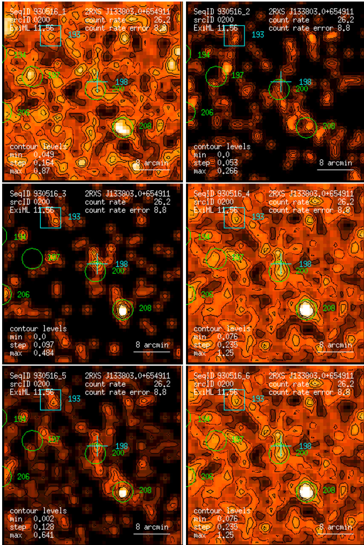
Figure 200: RASS 930516: detection 0200: band rate images, Gaussian filter: (1) PSPC channels 11 – 41, (2) 52 – 90, (3) 91 – 201, (4) 11 – 235, (5) 52 – 201, (6) 11 – 201. Broad band rates in counts/ks. Band rate contour levels in counts/ks/arcmin 2 .
