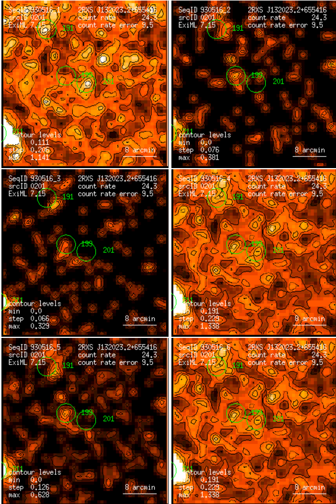
Figure 201: RASS 930516: detection 0201: band rate images, Gaussian filter: (1) PSPC channels 11 – 41, (2) 52 – 90, (3) 91 – 201, (4) 11 – 235, (5) 52 – 201, (6) 11 – 201. Broad band rates in counts/ks. Band rate contour levels in counts/ks/arcmin 2 .
