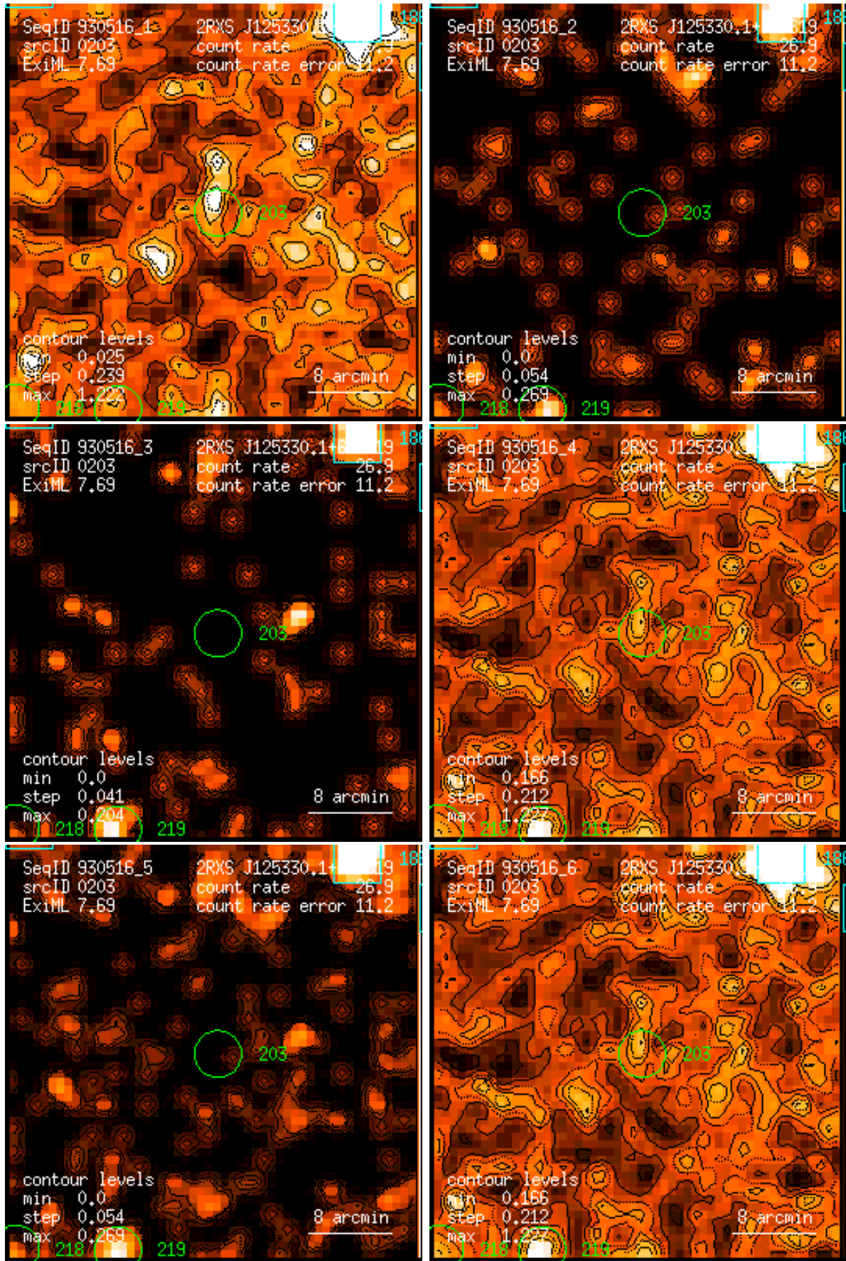
Figure 203: RASS 930516: detection 0203: band rate images, Gaussian filter: (1) PSPC channels 11 – 41, (2) 52 – 90, (3) 91 – 201, (4) 11 – 235, (5) 52 – 201, (6) 11 – 201. Broad band rates in counts/ks. Band rate contour levels in counts/ks/arcmin 2 .
