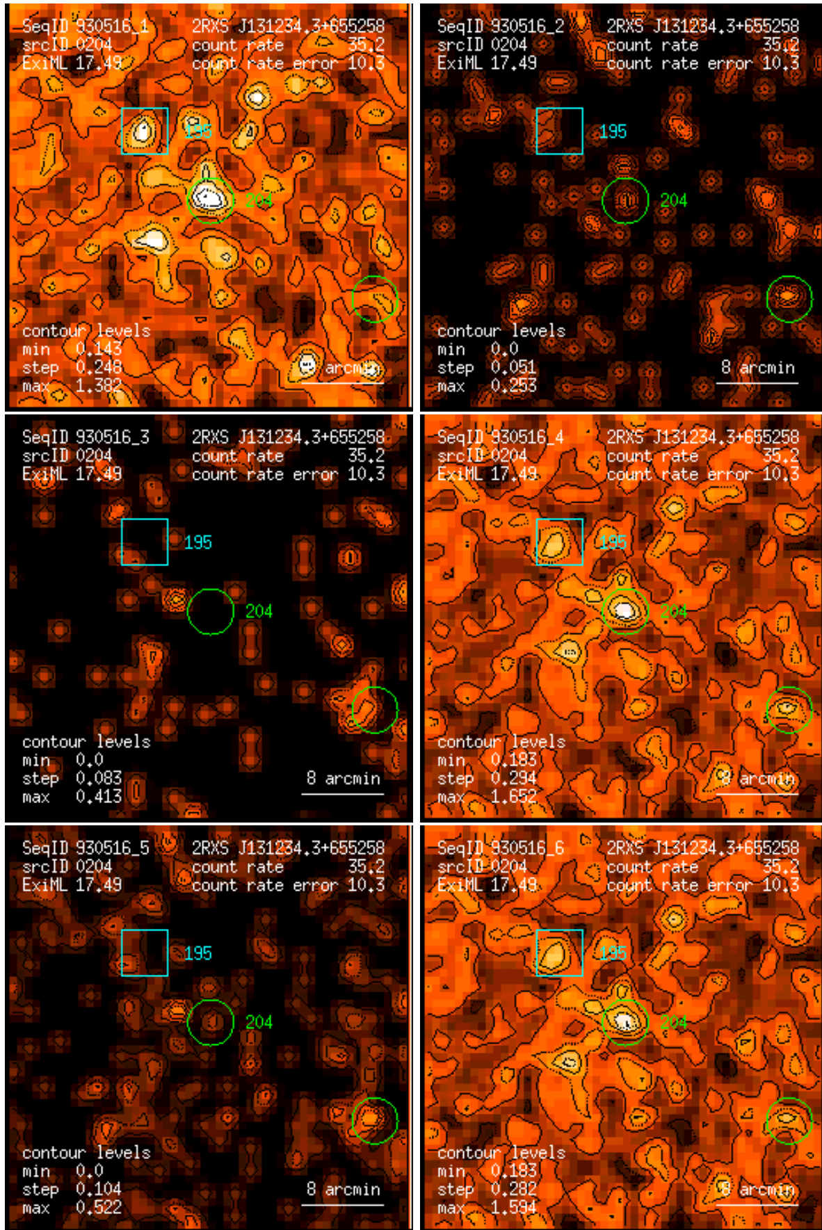
Figure 204: RASS 930516: detection 0204: band rate images, Gaussian filter: (1) PSPC channels 11 – 41, (2) 52 – 90, (3) 91 – 201, (4) 11 – 235, (5) 52 – 201, (6) 11 – 201. Broad band rates in counts/ks. Band rate contour levels in counts/ks/arcmin 2 .
