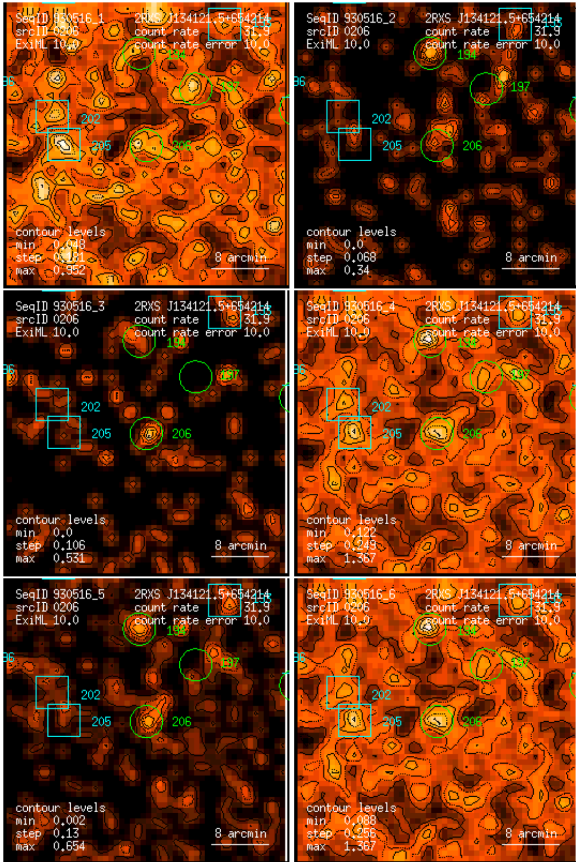
Figure 206: RASS 930516: detection 0206: band rate images, Gaussian filter: (1) PSPC channels 11 – 41, (2) 52 – 90, (3) 91 – 201, (4) 11 – 235, (5) 52 – 201, (6) 11 – 201. Broad band rates in counts/ks. Band rate contour levels in counts/ks/arcmin 2 .
