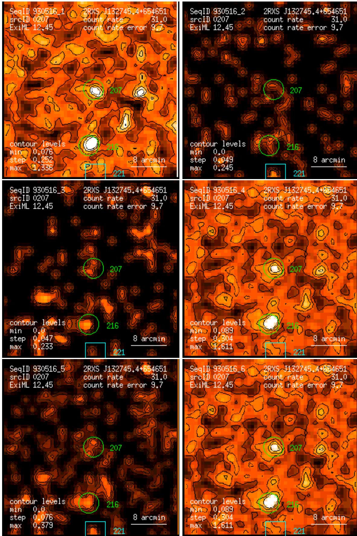
Figure 207: RASS 930516: detection 0207: band rate images, Gaussian filter: (1) PSPC channels 11 – 41, (2) 52 – 90, (3) 91 – 201, (4) 11 – 235, (5) 52 – 201, (6) 11 – 201. Broad band rates in counts/ks. Band rate contour levels in counts/ks/arcmin 2 .
