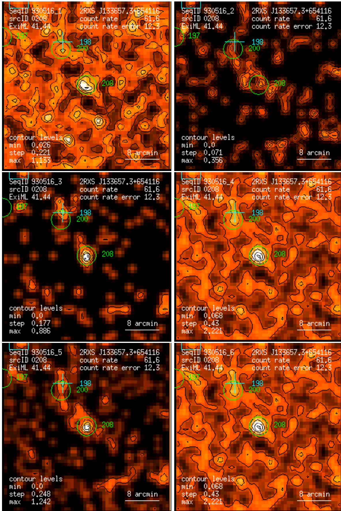
Figure 208: RASS 930516: detection 0208: band rate images, Gaussian filter: (1) PSPC channels 11 – 41, (2) 52 – 90, (3) 91 – 201, (4) 11 – 235, (5) 52 – 201, (6) 11 – 201. Broad band rates in counts/ks. Band rate contour levels in counts/ks/arcmin 2 .
