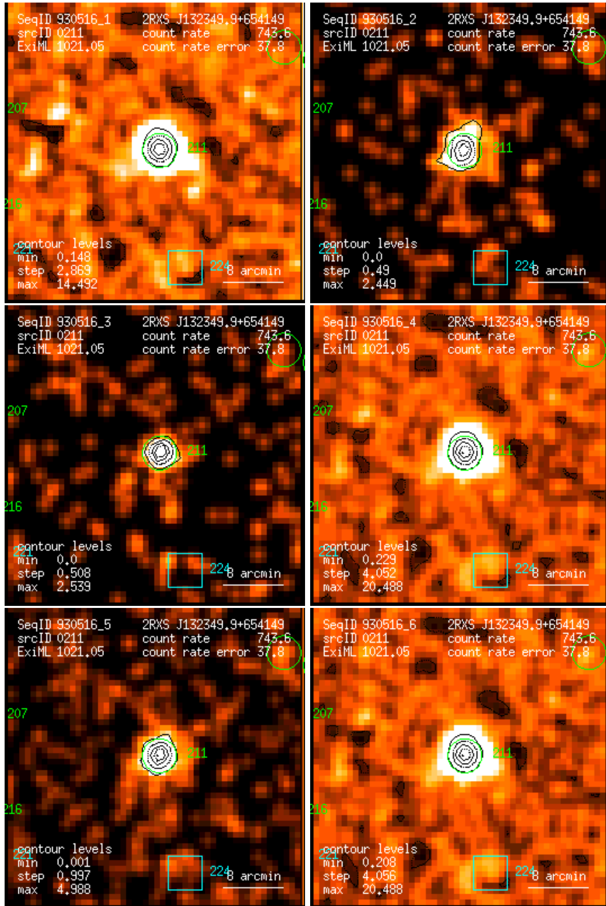
Figure 211: RASS 930516: detection 0211: band rate images, Gaussian filter: (1) PSPC channels 11 – 41, (2) 52 – 90, (3) 91 – 201, (4) 11 – 235, (5) 52 – 201, (6) 11 – 201. Broad band rates in counts/ks. Band rate contour levels in counts/ks/arcmin 2 .
