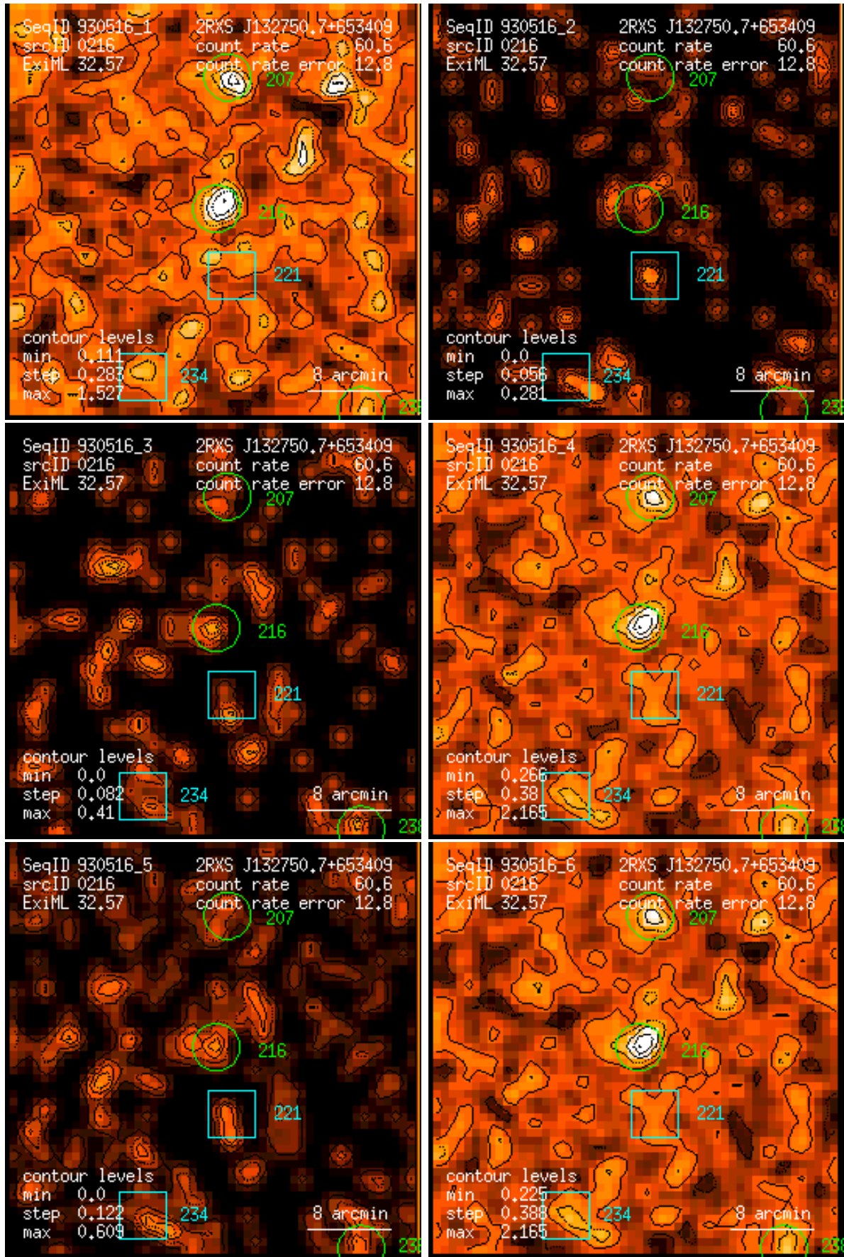
Figure 216: RASS 930516: detection 0216: band rate images, Gaussian filter: (1) PSPC channels 11 – 41, (2) 52 – 90, (3) 91 – 201, (4) 11 – 235, (5) 52 – 201, (6) 11 – 201. Broad band rates in counts/ks. Band rate contour levels in counts/ks/arcmin 2 .
