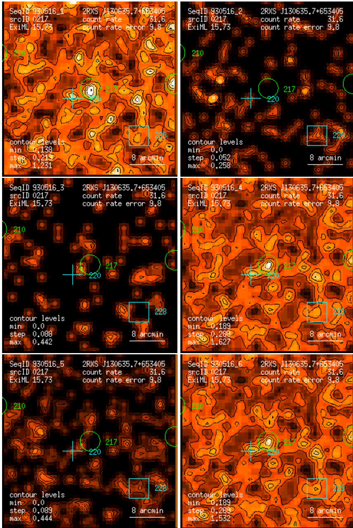
Figure 217: RASS 930516: detection 0217: band rate images, Gaussian filter: (1) PSPC channels 11 – 41, (2) 52 – 90, (3) 91 – 201, (4) 11 – 235, (5) 52 – 201, (6) 11 – 201. Broad band rates in counts/ks. Band rate contour levels in counts/ks/arcmin 2 .
