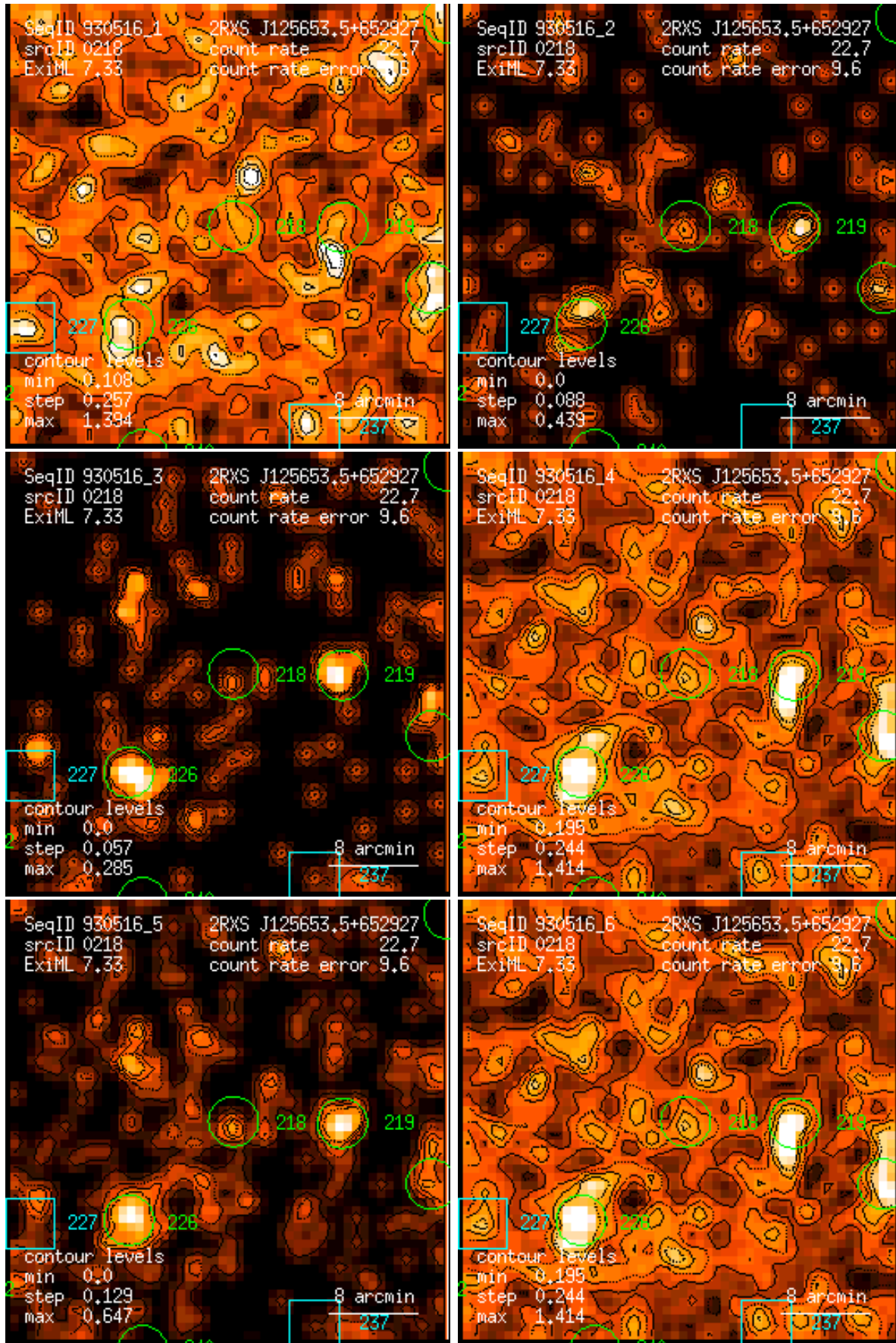
Figure 218: RASS 930516: detection 0218: band rate images, Gaussian filter: (1) PSPC channels 11 – 41, (2) 52 – 90, (3) 91 – 201, (4) 11 – 235, (5) 52 – 201, (6) 11 – 201. Broad band rates in counts/ks. Band rate contour levels in counts/ks/arcmin 2 .
