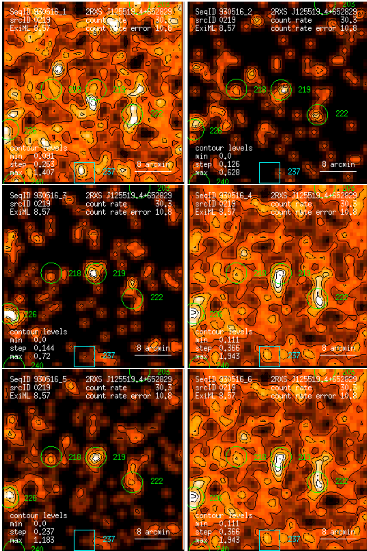
Figure 219: RASS 930516: detection 0219: band rate images, Gaussian filter: (1) PSPC channels 11 – 41, (2) 52 – 90, (3) 91 – 201, (4) 11 – 235, (5) 52 – 201, (6) 11 – 201. Broad band rates in counts/ks. Band rate contour levels in counts/ks/arcmin 2 .
