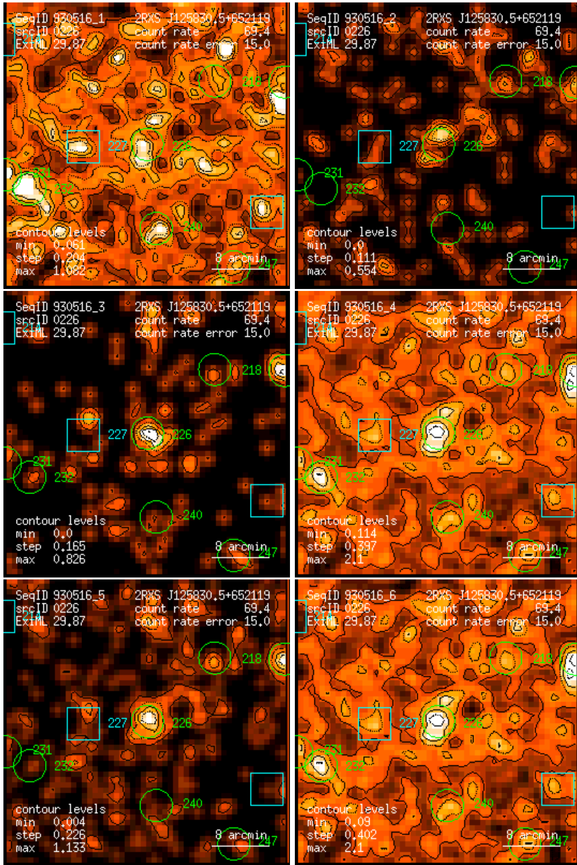
Figure 226: RASS 930516: detection 0226: band rate images, Gaussian filter: (1) PSPC channels 11 – 41, (2) 52 – 90, (3) 91 – 201, (4) 11 – 235, (5) 52 – 201, (6) 11 – 201. Broad band rates in counts/ks. Band rate contour levels in counts/ks/arcmin 2 .
