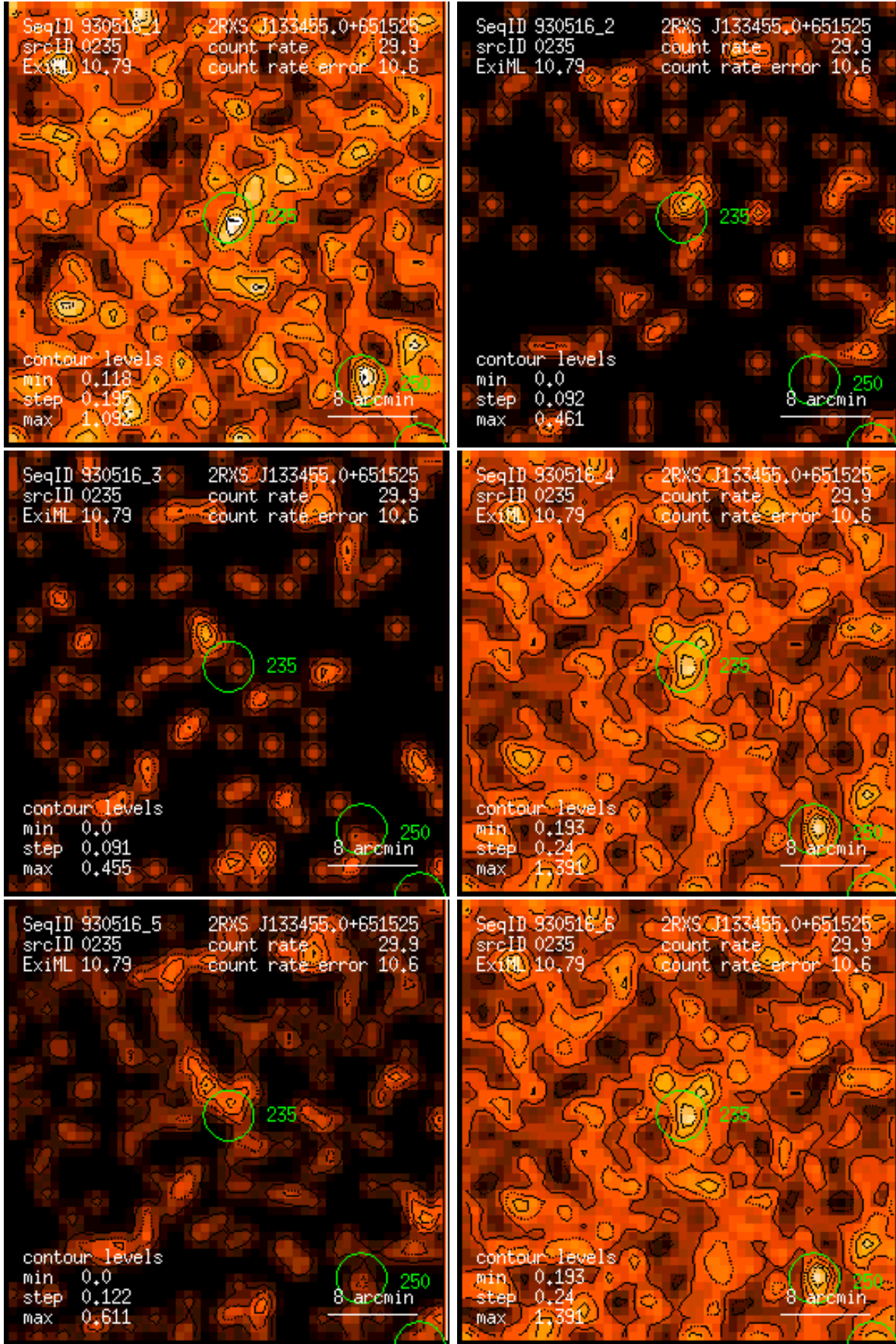
Figure 235: RASS 930516: detection 0235: band rate images, Gaussian filter: (1) PSPC channels 11 – 41, (2) 52 – 90, (3) 91 – 201, (4) 11 – 235, (5) 52 – 201, (6) 11 – 201. Broad band rates in counts/ks. Band rate contour levels in counts/ks/arcmin 2 .
